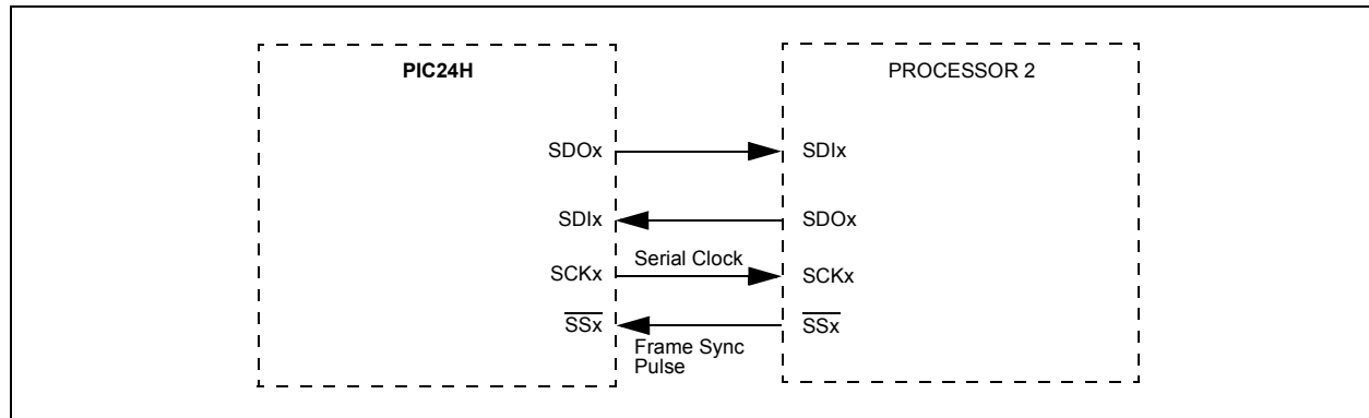
FIGURE 14-4: SPI MASTER AND FRAME SLAVE CONNECTION DIAGRAM
