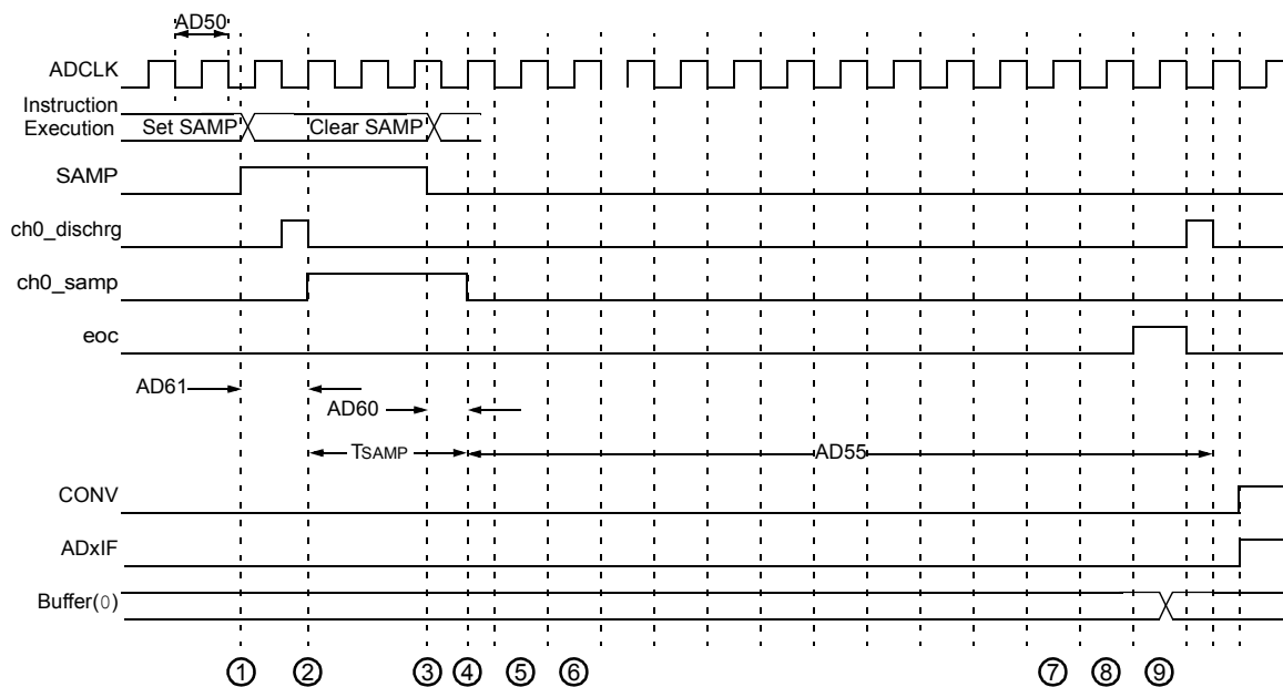
FIGURE 23-18: ADC CONVERSION (12-BIT MODE) TIMING CHARACTERISTICS (ASAM = 0, SSRC<2:0> = 000)
