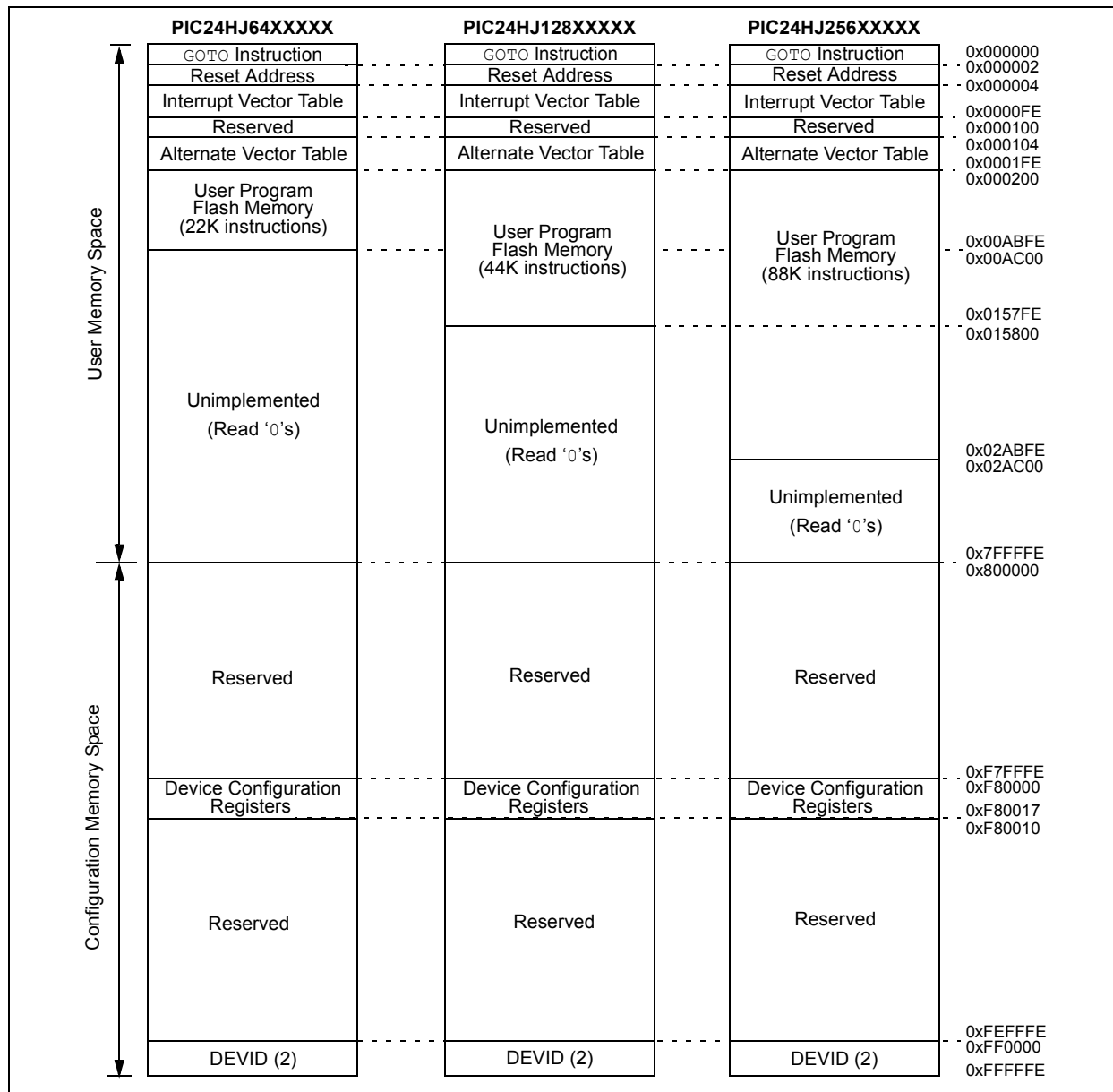
FIGURE 3-1: PROGRAM MEMORY MAP FOR PIC24HJXXXGPX06/X08/X10 FAMILY DEVICES
