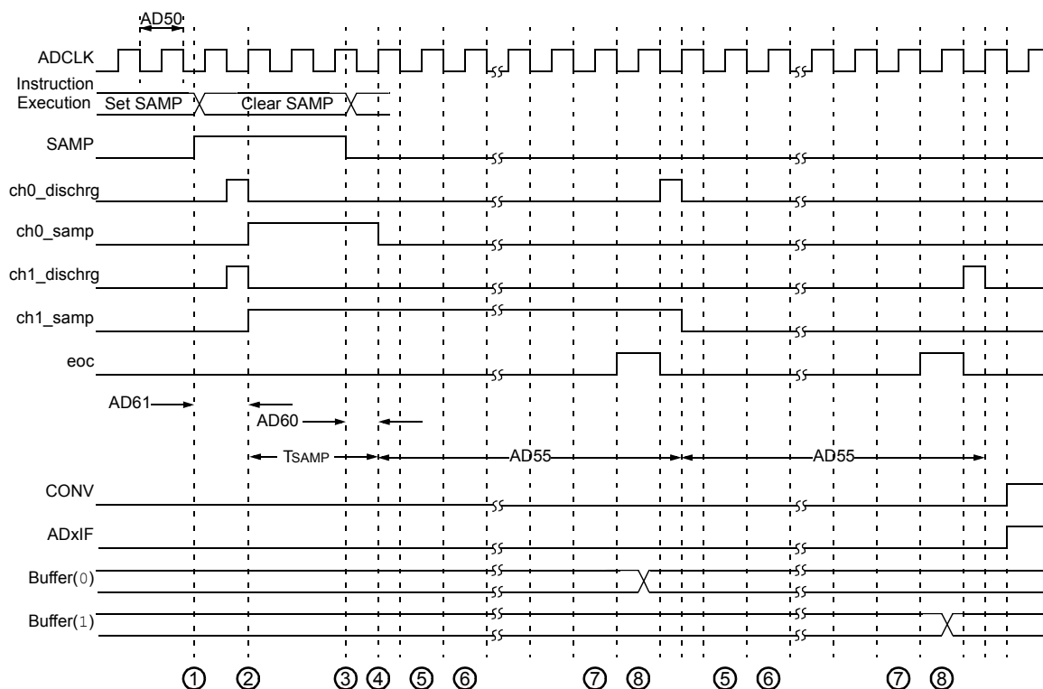
FIGURE 23-19: ADC CONVERSION (10-BIT MODE) TIMING CHARACTERISTICS (CHPS<1:0> = 01, SIMSAM = 0, ASAM = 0, SSRC<2:0> = 000)
