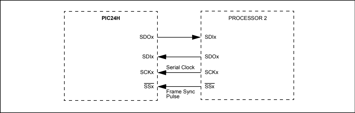
FIGURE 15-6: SPI SLAVE, FRAME SLAVE CONNECTION DIAGRAM
