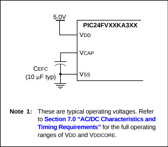
FIGURE 2-2: CONNECTIONS FOR THE ON-CHIP REGULATOR
