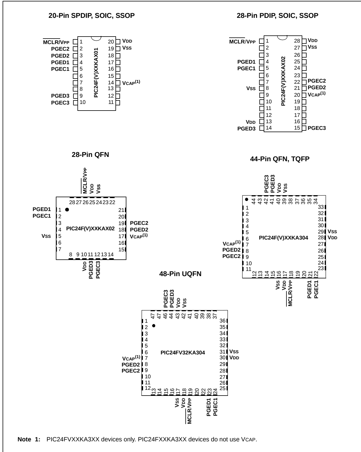
FIGURE 2-3: PIN DIAGRAMS
