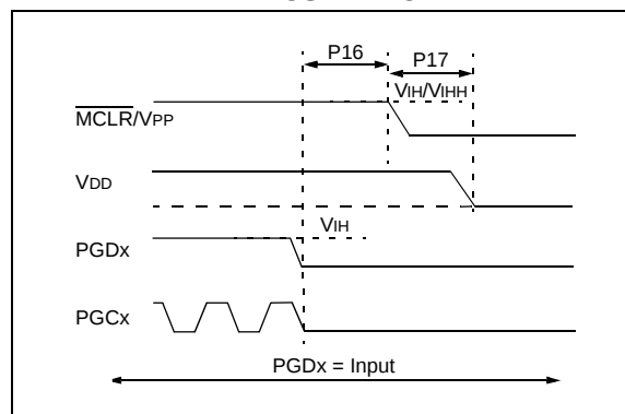
FIGURE 4-8: EXITING ENHANCED ICSP™ MODE
