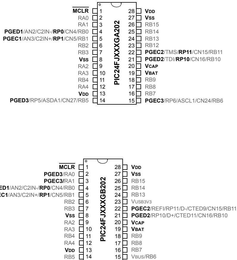
FIGURE 2-3: PIN DIAGRAMS (28-PIN PDIP/SSOP/SOIC)
