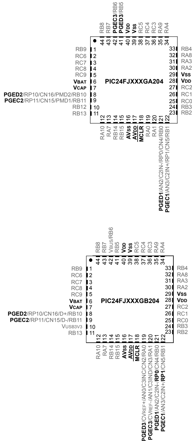
FIGURE 2-5: PIN DIAGRAMS (44-PIN QFN) (1)
