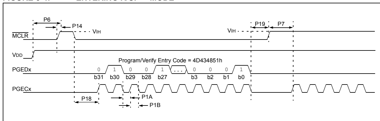
FIGURE 3-4: ENTERING ICSP™ MODE
