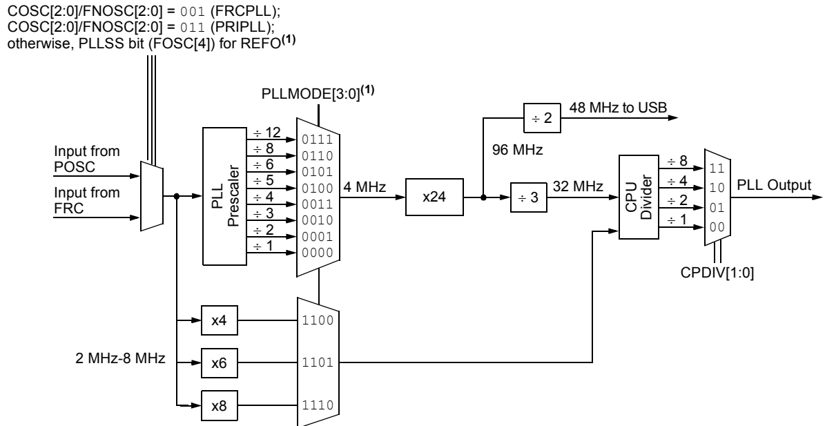
Figure 9-2. PLL Block
