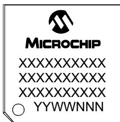
64-Lead QFN (9x9x0.9 mm)
