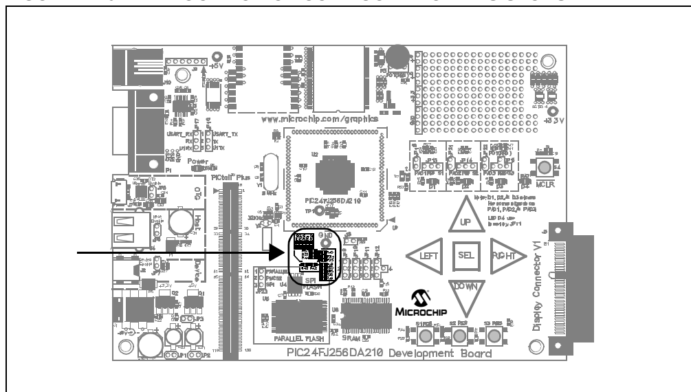
FIGURE 4-10: LOCATION OF CONFIGURATION RESISTORS
