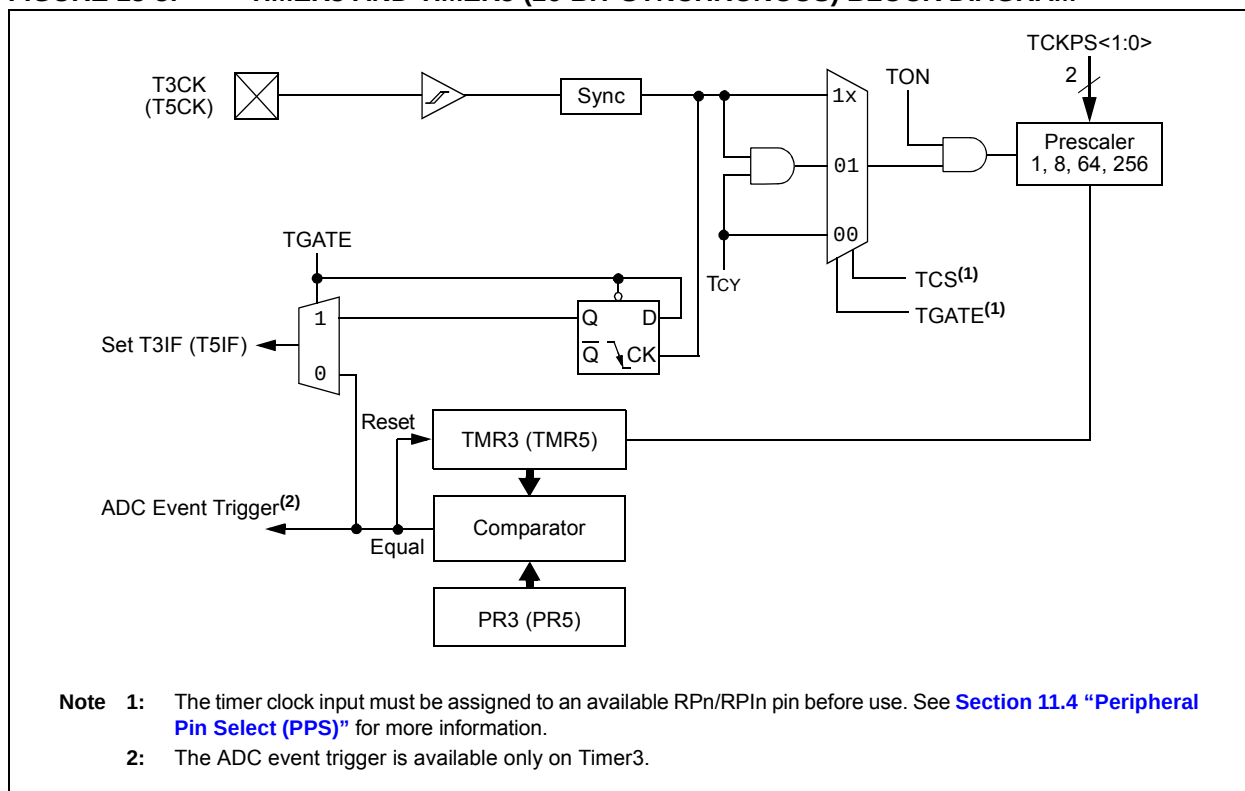
FIGURE 13-3: TIMER3 AND TIMER5 (16-BIT SYNCHRONOUS) BLOCK DIAGRAM
