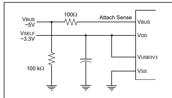
FIGURE 20-3: SELF-POWER ONLY
