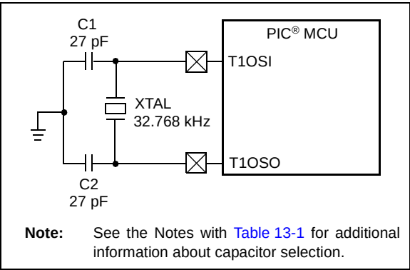
FIGURE 13-4: EXTERNAL COMPONENTS FOR THE TIMER1 LP OSCILLATOR
