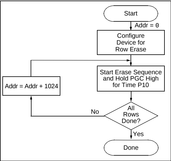
FIGURE 3-3: ROW ERASE CODE MEMORY FLOW
