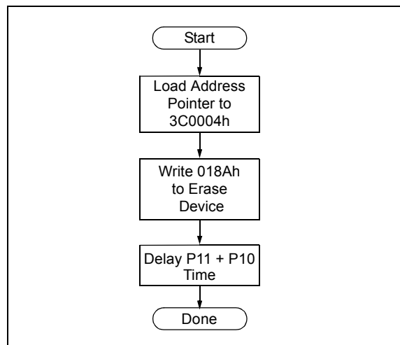
FIGURE 3-2: CHIP ERASE FLOW
