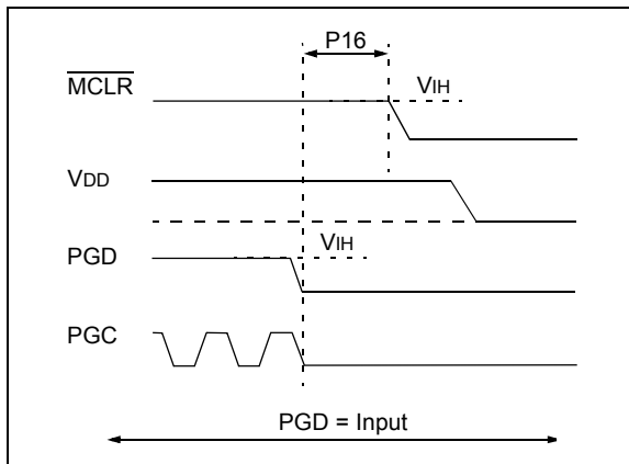
FIGURE 2-11: EXITING PROGRAM/VERIFY MODE
