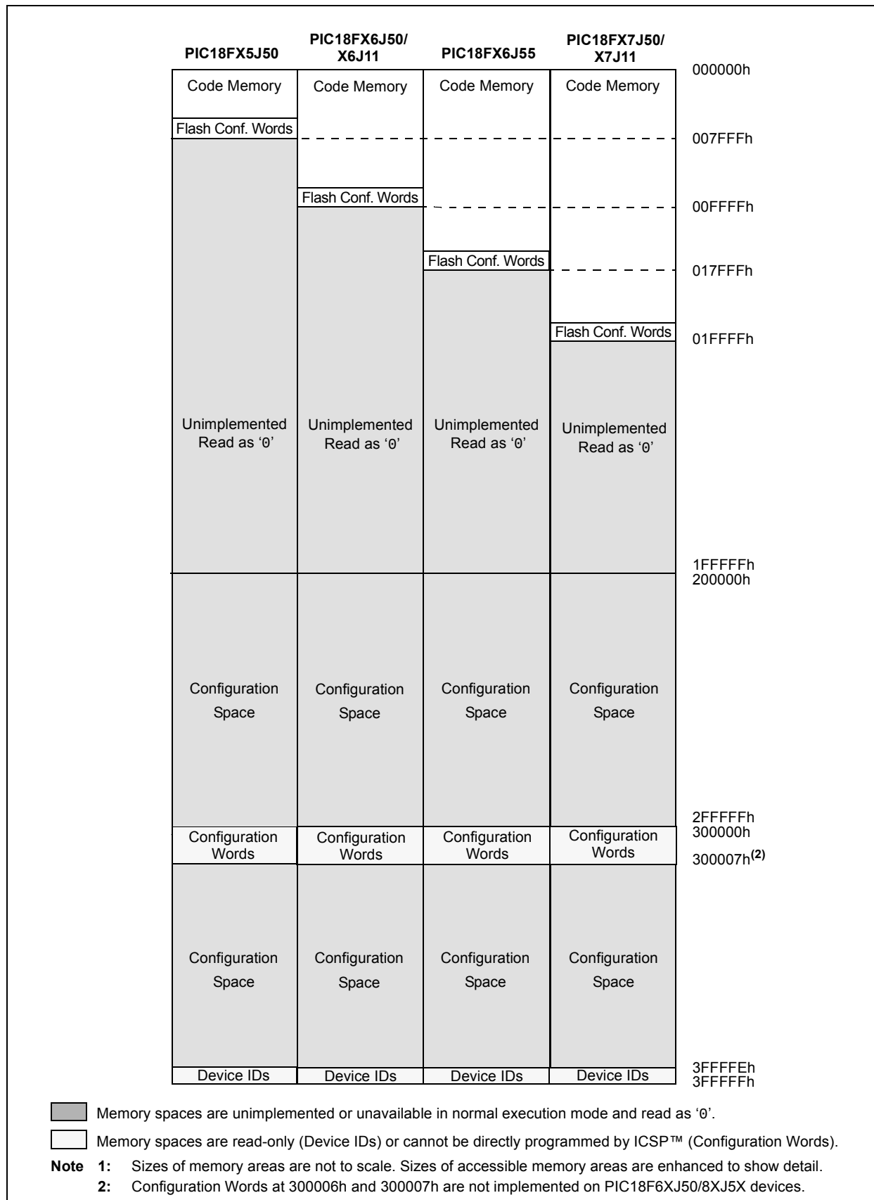
FIGURE 2-7: MEMORY MAPS FOR PIC18F6XJ5X/8XJ5X DEVICES (1)
