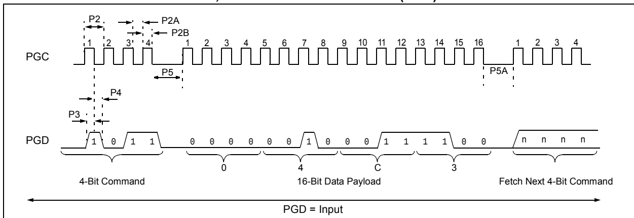
FIGURE 2-12: TABLE WRITE, POST-INCREMENT TIMING (1101)
