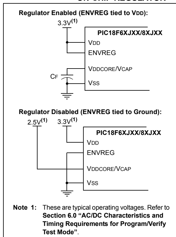
FIGURE 2-4: CONNECTIONS FOR THE ON-CHIP REGULATOR
