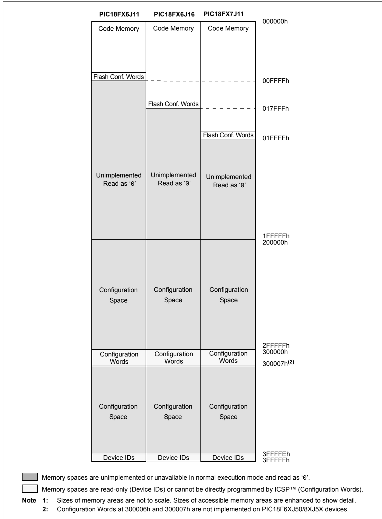
FIGURE 2-8: MEMORY MAPS FOR PIC18F6XJ11/F6XJ16/F8XJ11/F8XJ16 DEVICES (1)
