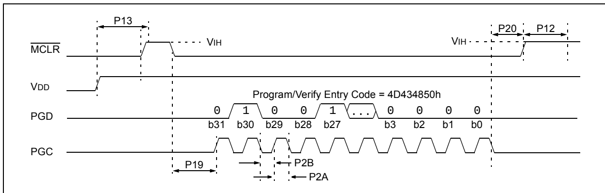
FIGURE 2-10: ENTERING PROGRAM/VERIFY MODE
