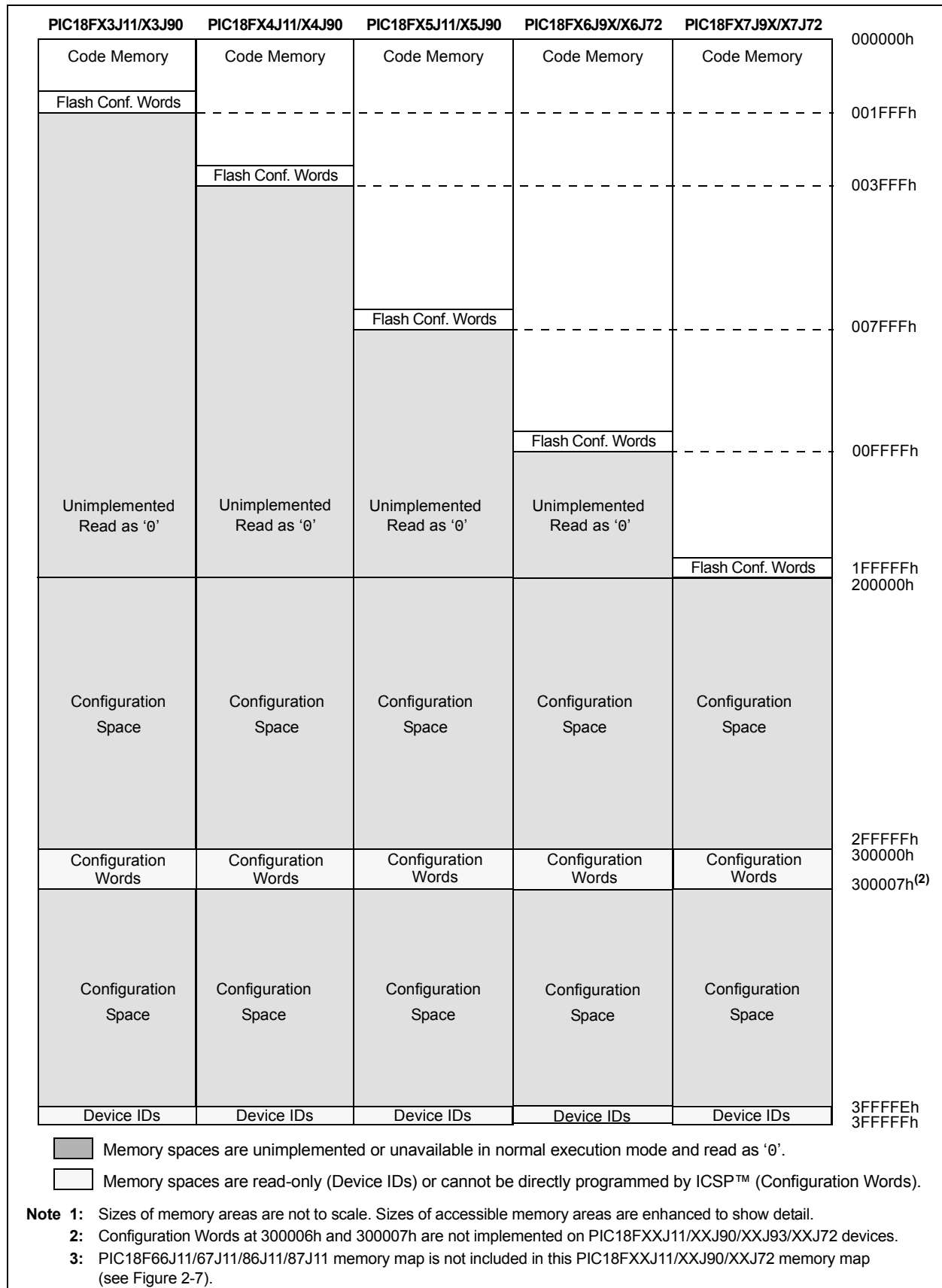
FIGURE 2-6: MEMORY MAPS FOR PIC18FXXJ11/XXJ9X/XXJ72 DEVICES (1)
