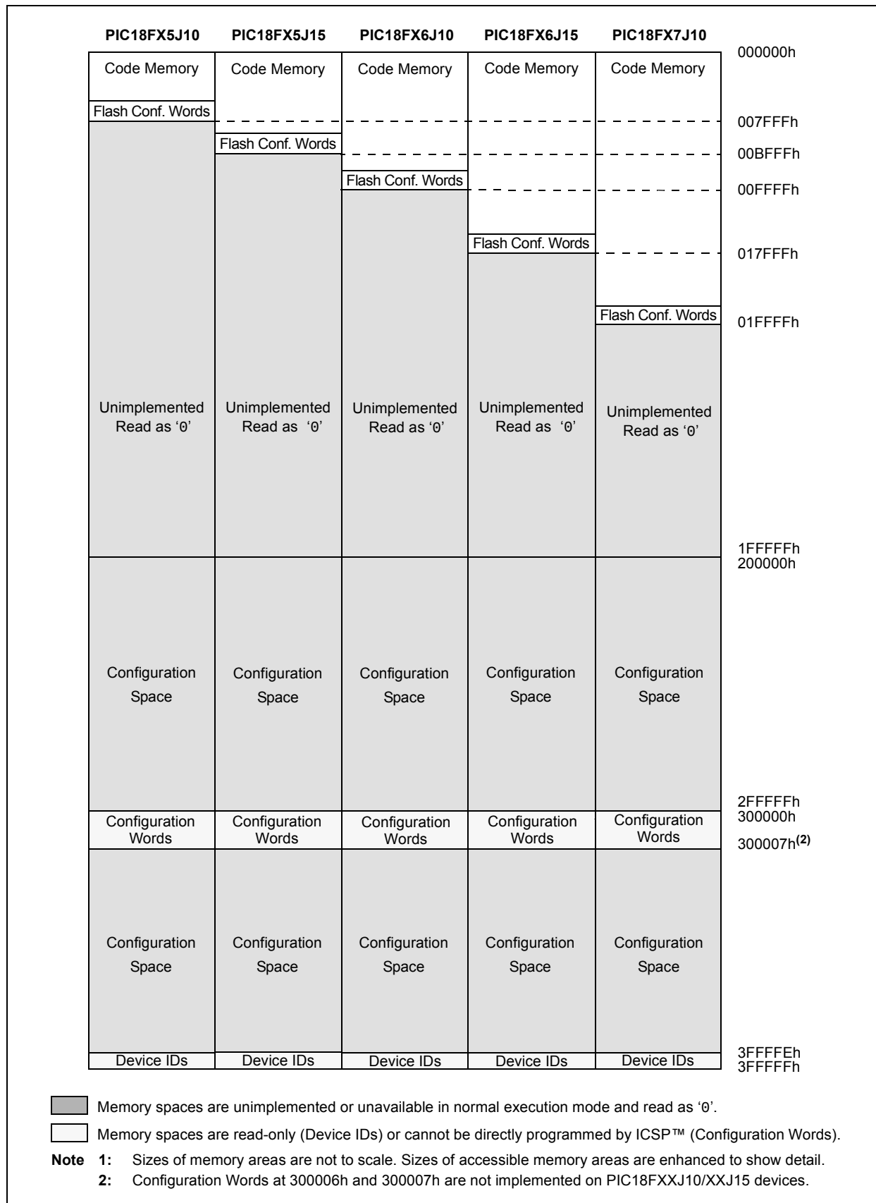
FIGURE 2-5: MEMORY MAPS FOR PIC18FXXJ10/XXJ15 DEVICES (1)
