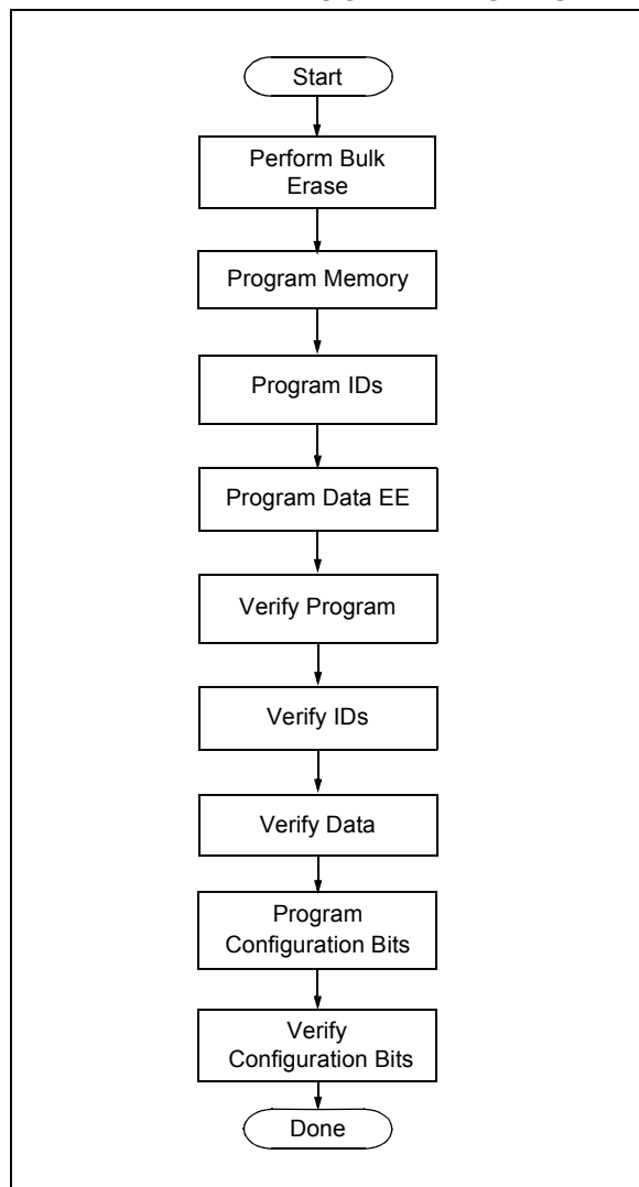
FIGURE 2-6: HIGH-LEVEL PROGRAMMING FLOW
