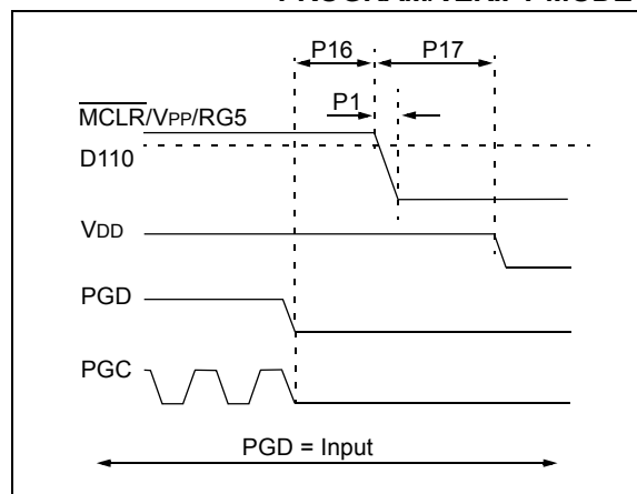
FIGURE 2-8: EXITING HIGH-VOLTAGE PROGRAM/VERIFY MODE
