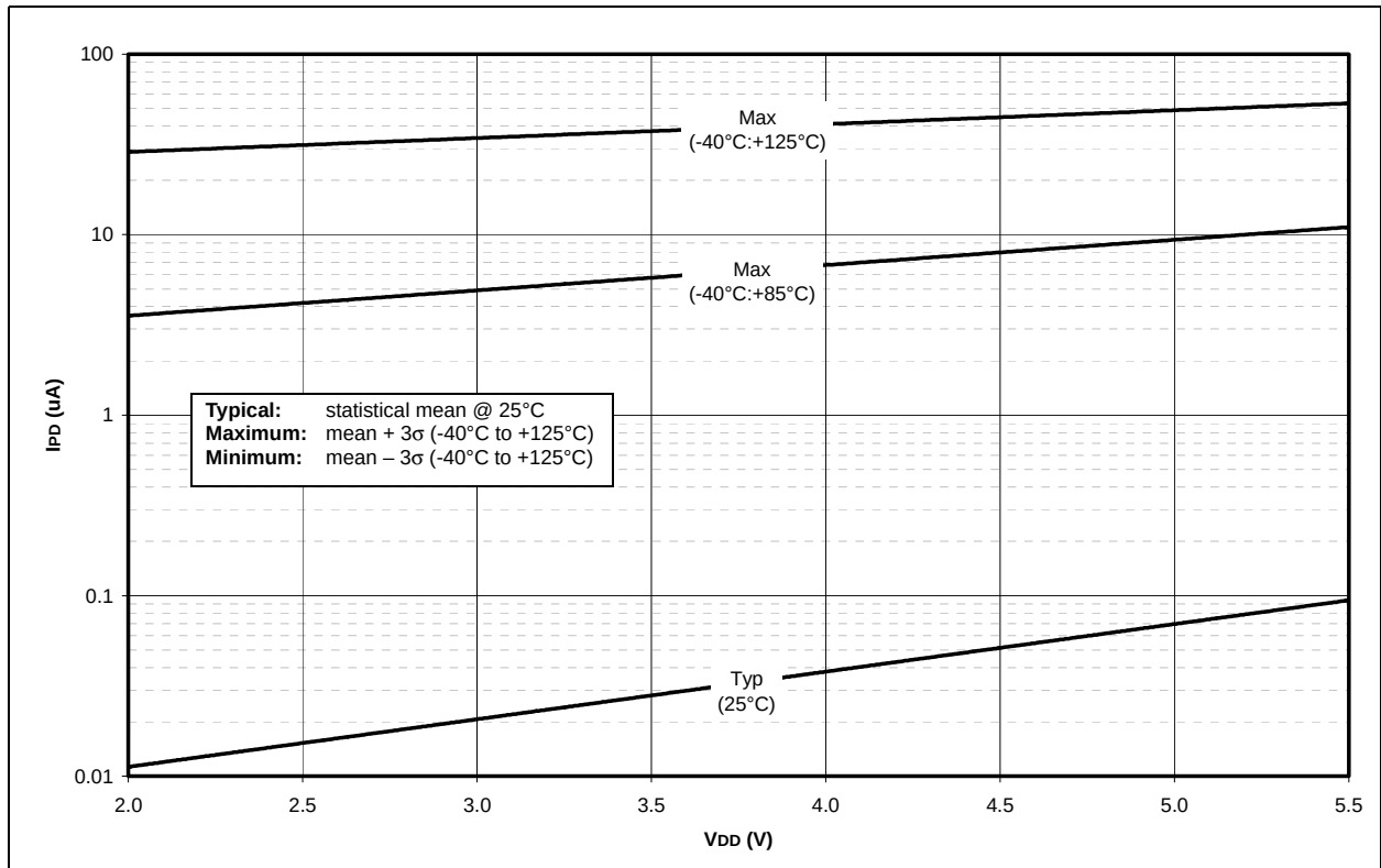
FIGURE 27-14: MAXIMUM I_{PD} vs. V_{DD} OVER TEMPERATURE
