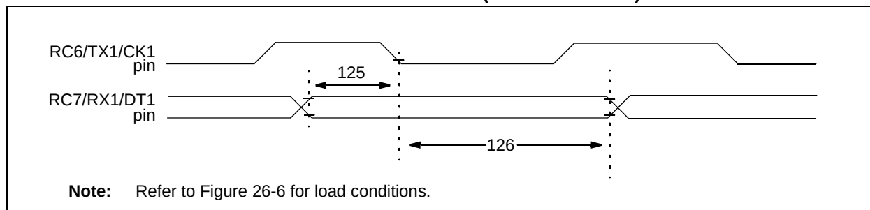
FIGURE 26-25: USART SYNCHRONOUS RECEIVE (MASTER/SLAVE) TIMING
