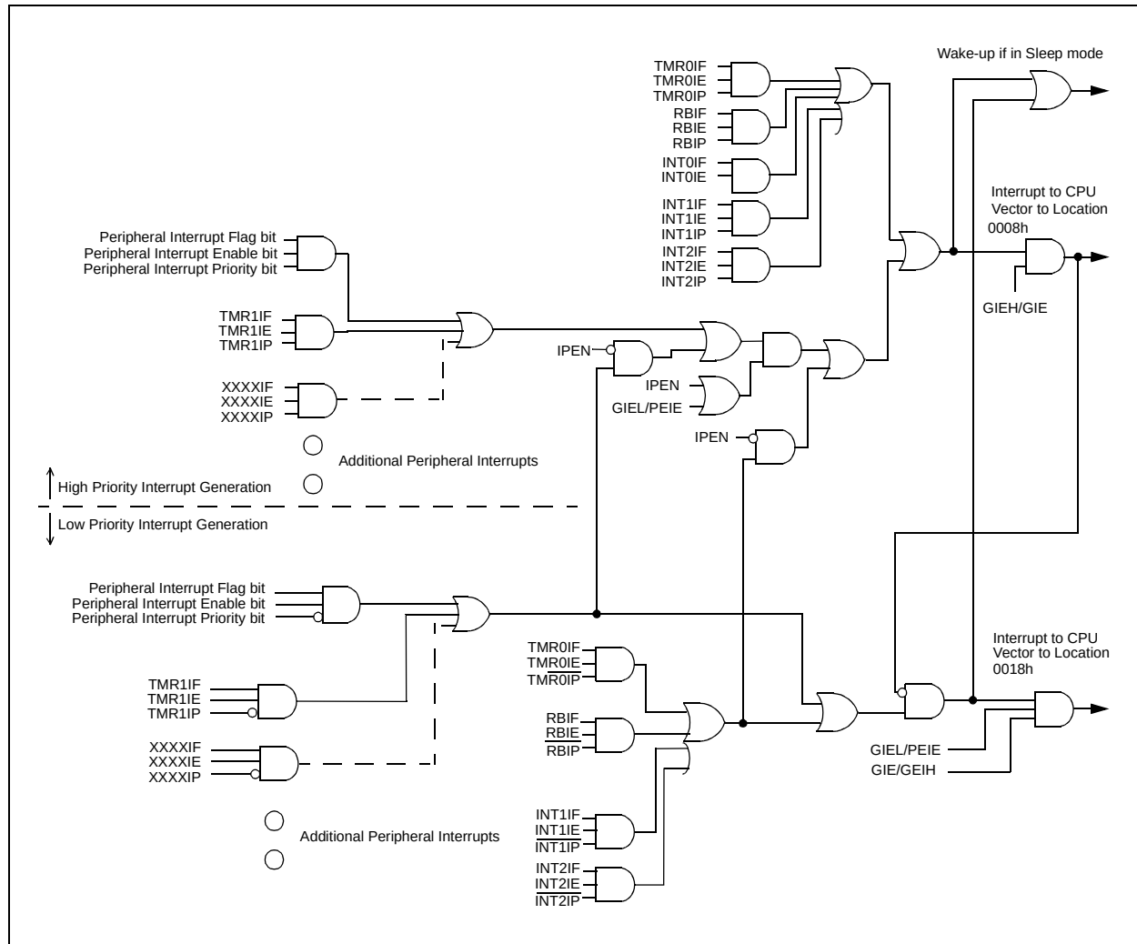
FIGURE 9-1: INTERRUPT LOGIC
