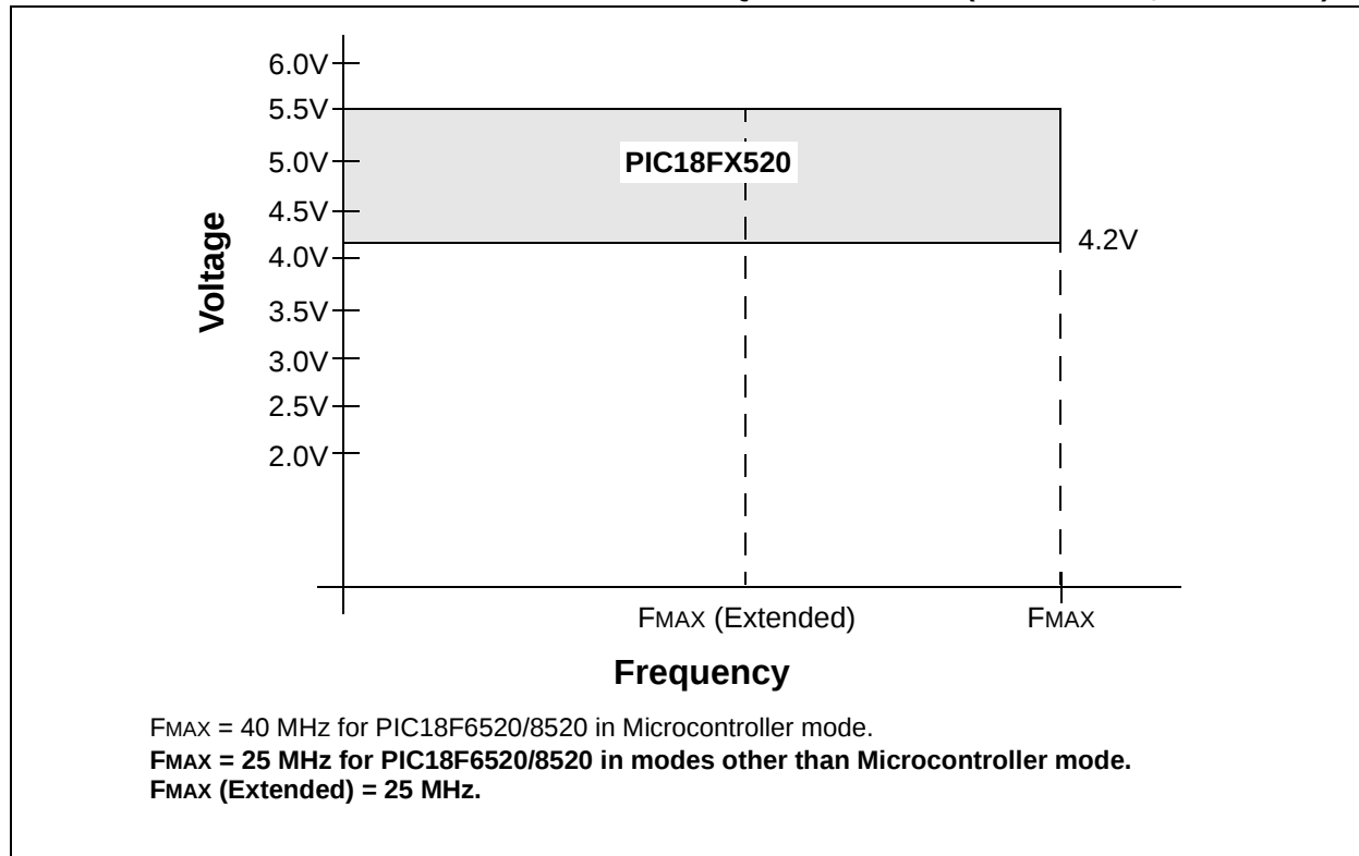
FIGURE 26-1: PIC18F6520/8520 VOLTAGE-FREQUENCY GRAPH (INDUSTRIAL, EXTENDED)
