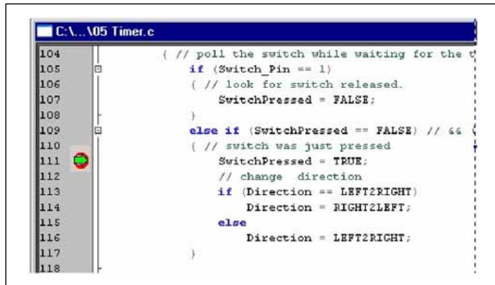
FIGURE 3-33: BREAKPOINT HALT
