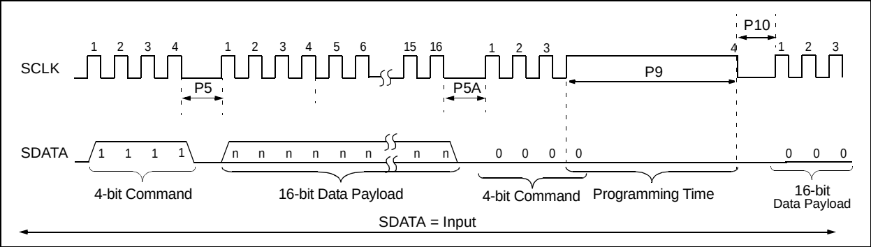
FIGURE 3-6: TABLE WRITE AND START PROGRAMMING INSTRUCTION TIMING (1111)
