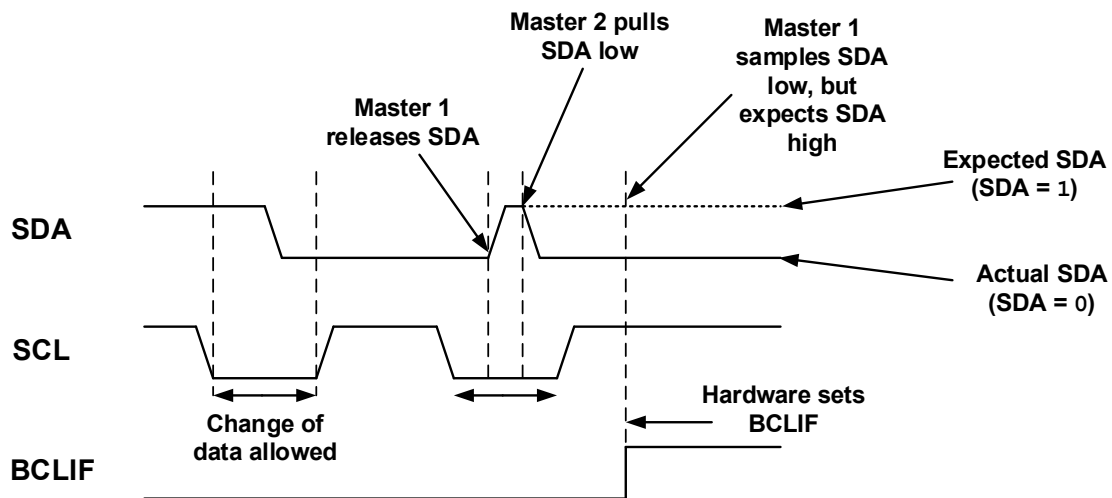
Figure 36-41. Bus Collision
