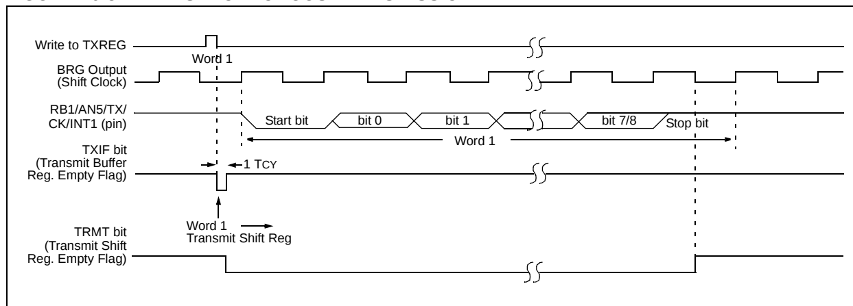
FIGURE 16-3: ASYNCHRONOUS TRANSMISSION
