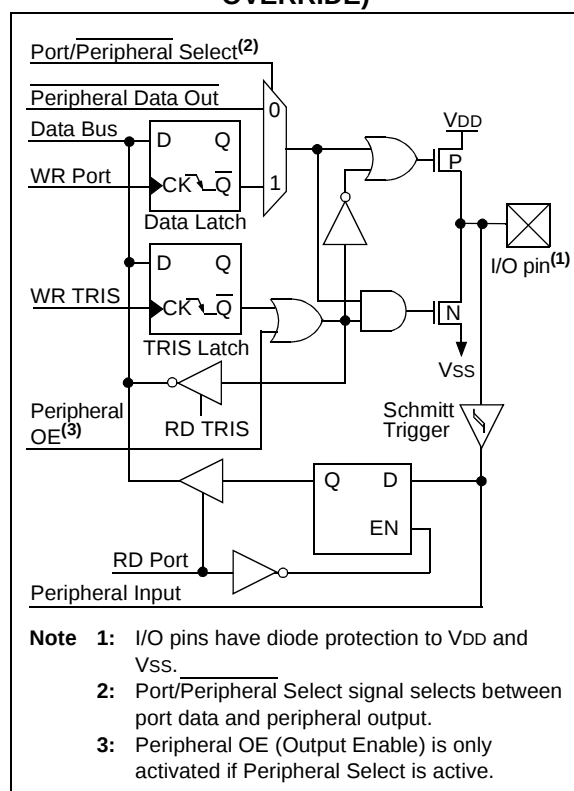
FIGURE 1: PORTC BLOCK DIAGRAM (PERIPHERAL OUTPUT OVERRIDE)
