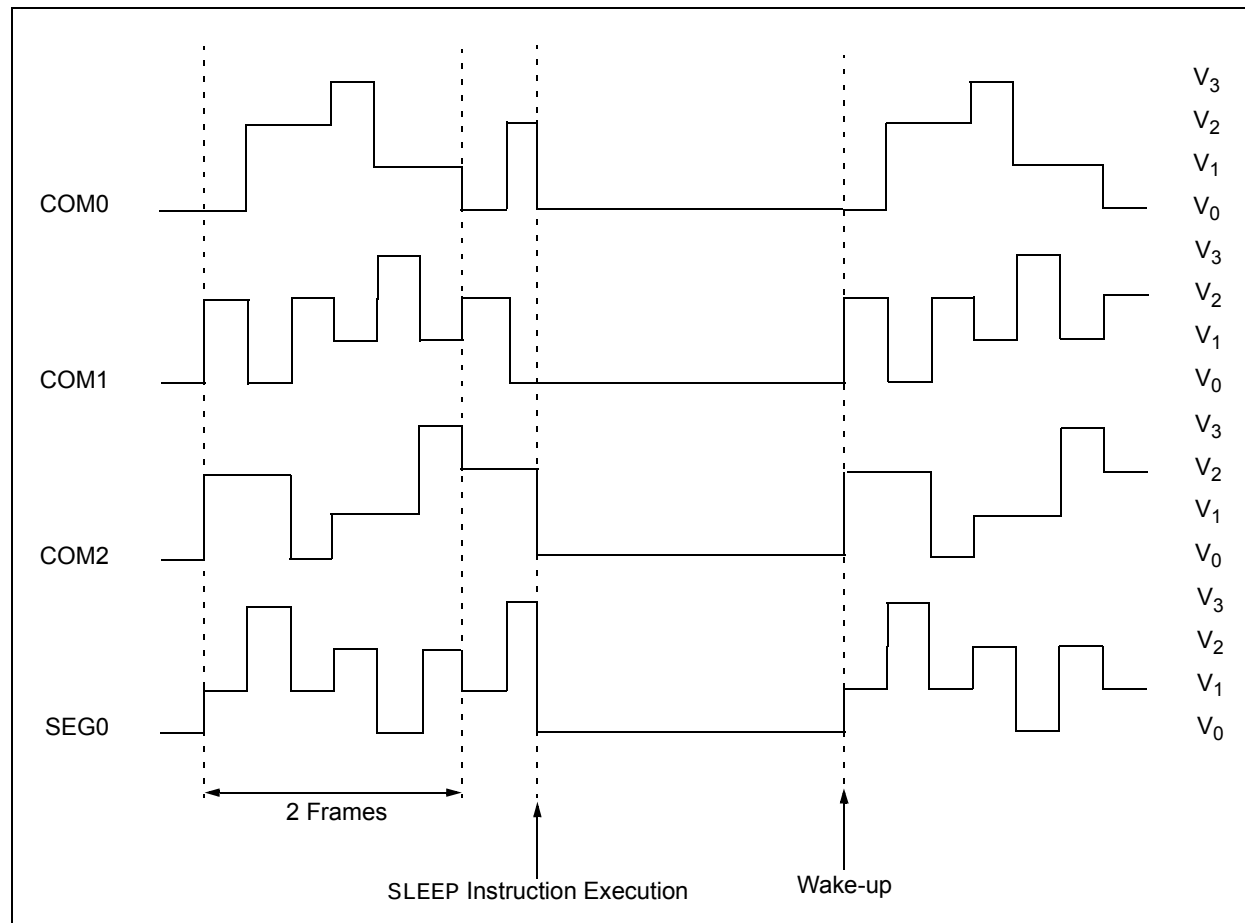
FIGURE 19-20: SLEEP ENTRY/EXIT WHEN SLPEN = 1
