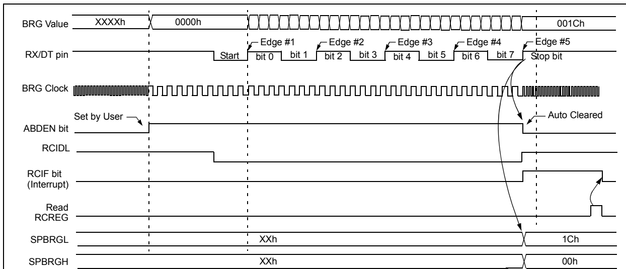
FIGURE 18-6: AUTOMATIC BAUD RATE CALIBRATION
