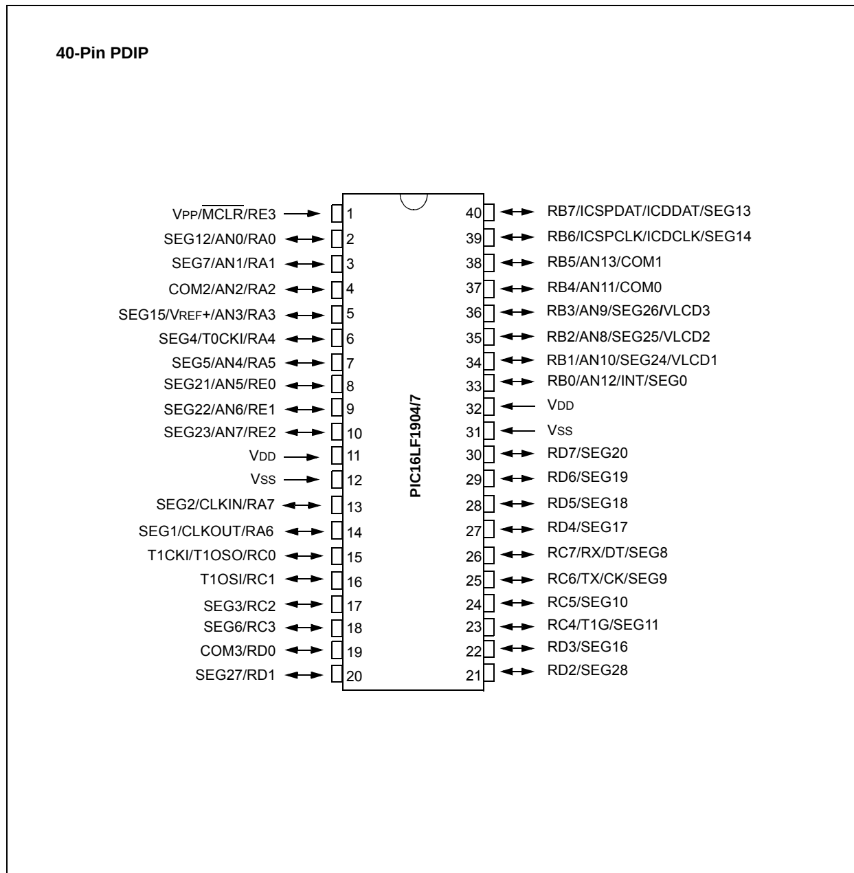
FIGURE 3: 40-PIN PDIP PACKAGE DIAGRAM FOR PIC16LF1904/7
