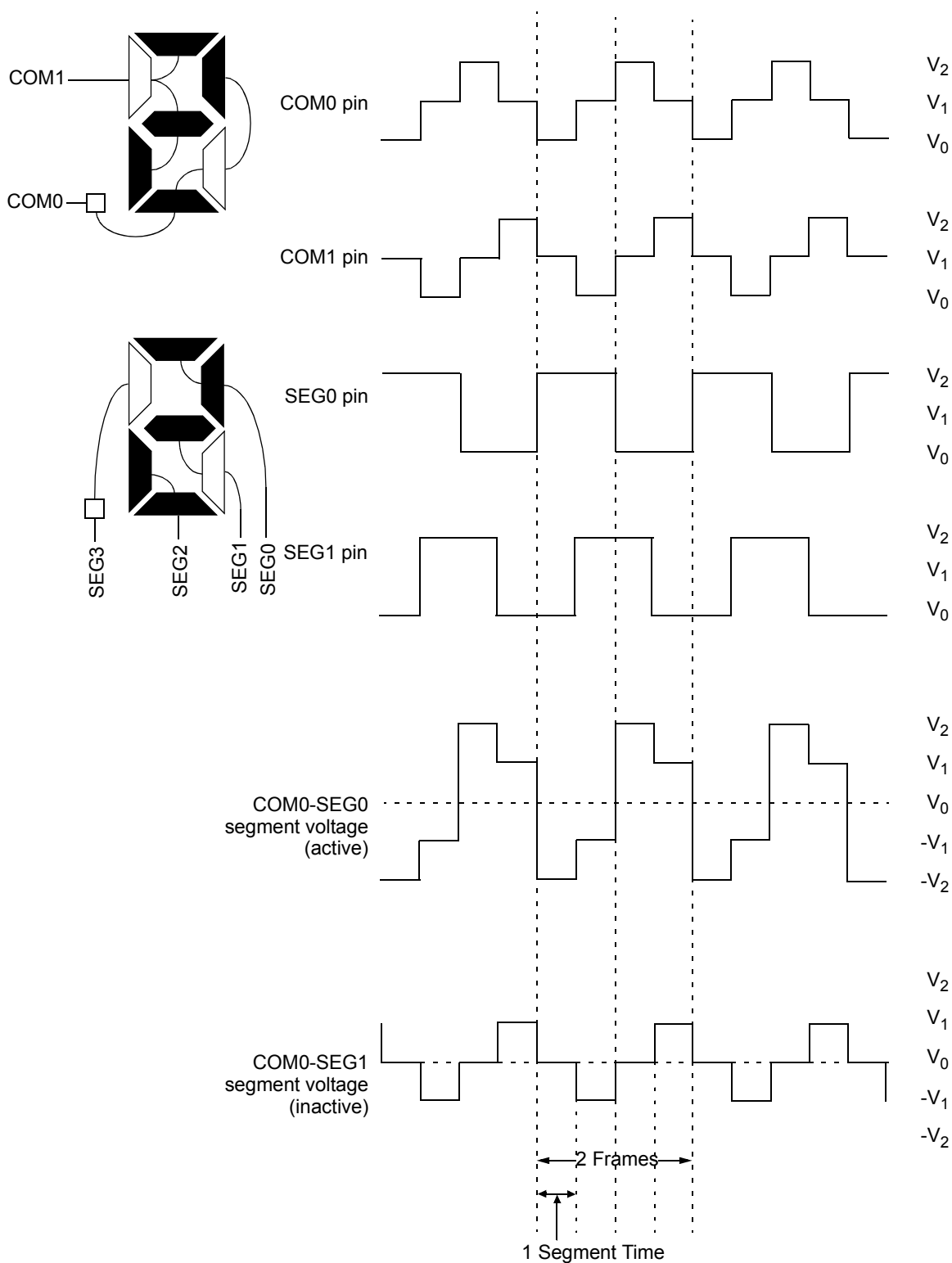
FIGURE 19-10: TYPE-B WAVEFORMS IN 1/2 MUX, 1/2 BIAS DRIVE
