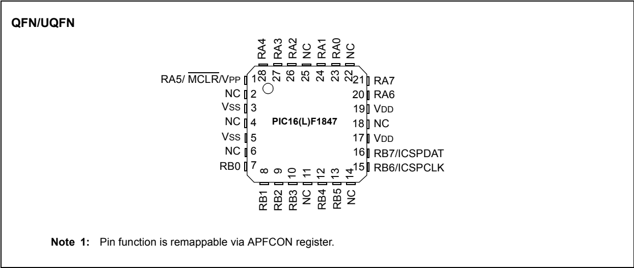
FIGURE 3: 28-PIN DIAGRAM FOR PIC16(L)F1847
