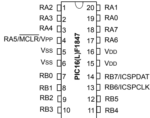
FIGURE 2: 20-PIN DIAGRAM FOR PIC16(L)F1847
