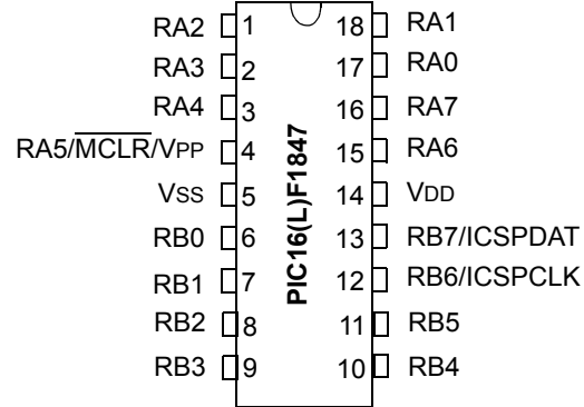
FIGURE 1: 18-PIN DIAGRAM FOR PIC16(L)F1847
