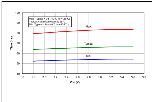
FIGURE 26-21: PWRT Period
