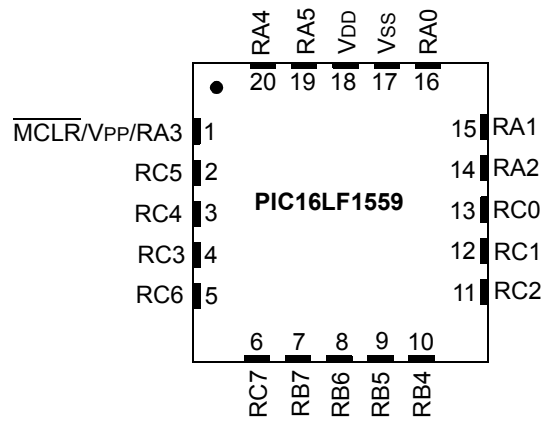
FIGURE 4: 20-PIN QFN,UQFN (4x4)
