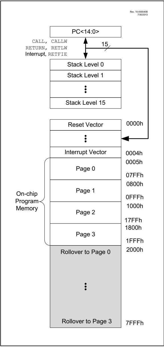
FIGURE 3-2: PROGRAM MEMORY MAP AND STACK FOR PIC16LF1559
