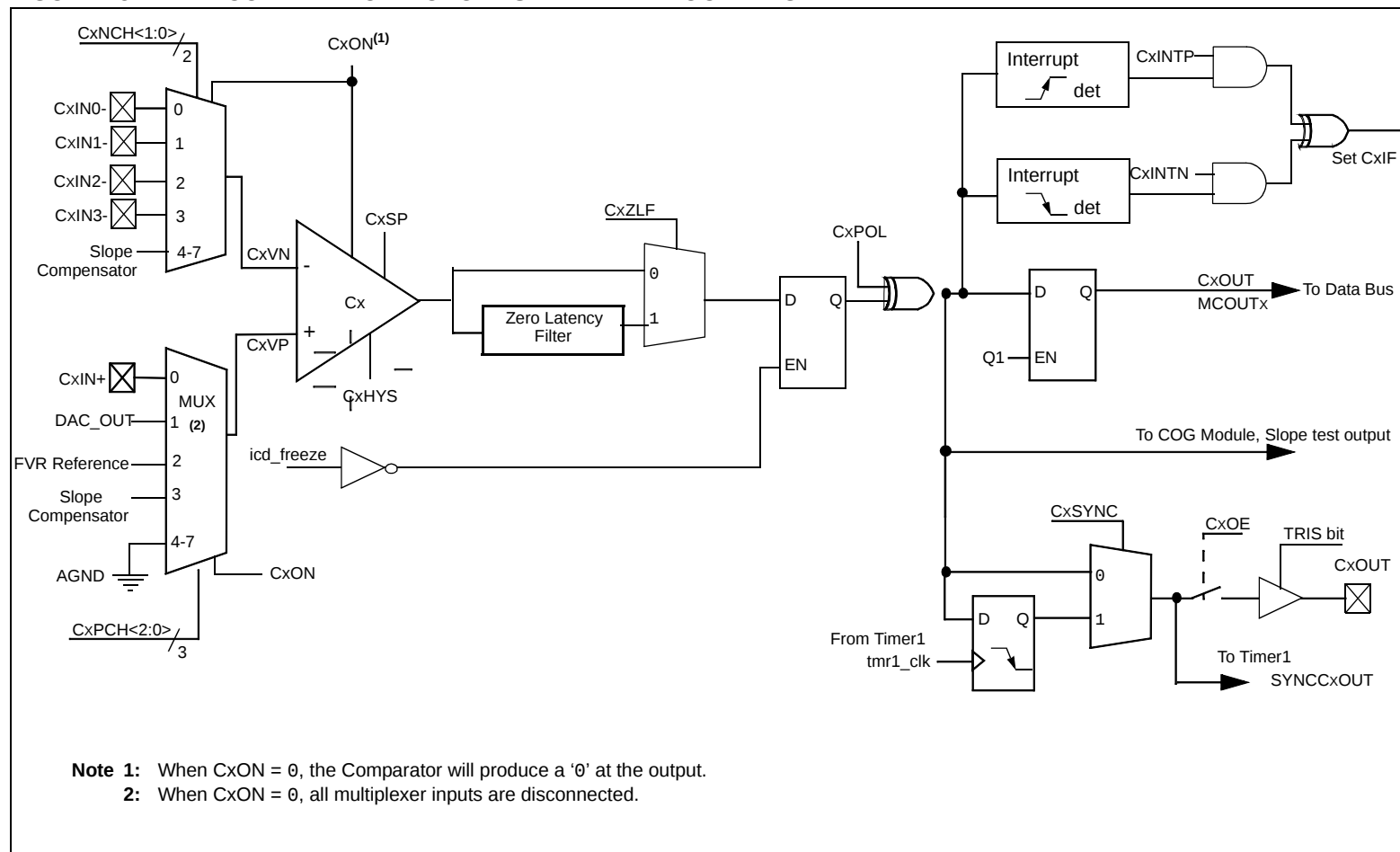
FIGURE 15-2: COMPARATOR MODULE SIMPLIFIED BLOCK DIAGRAM
