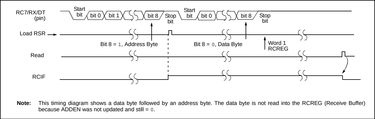
FIGURE 10-8: ASYNCHRONOUS RECEPTION WITH ADDRESS BYTE FIRST
