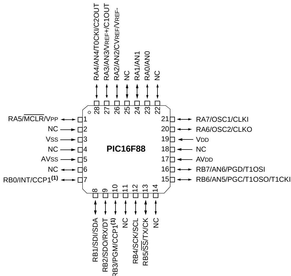
FIGURE 2-6: PIC16F88 28-PIN QFN
