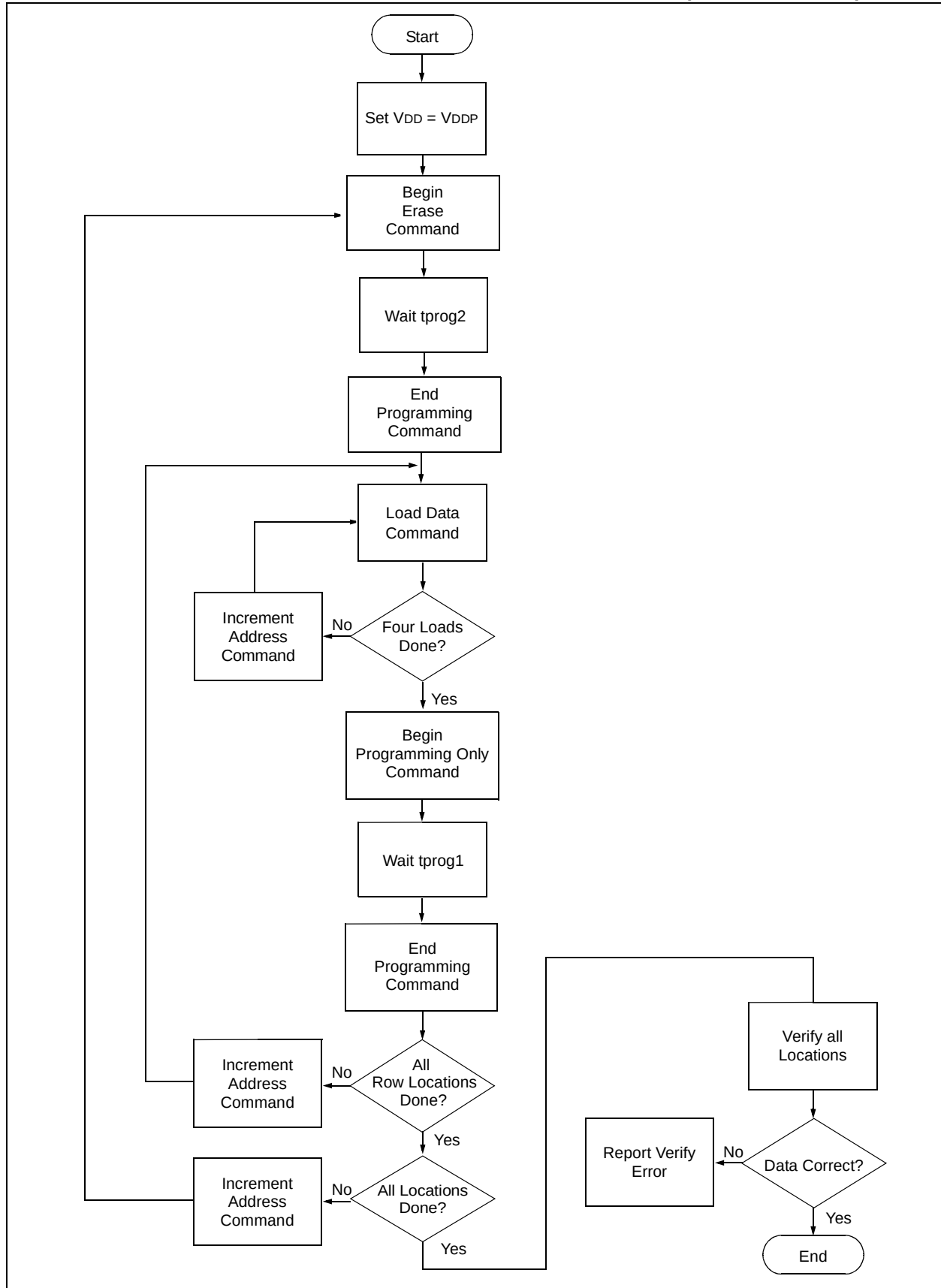
FIGURE 3-2: ALGORITHM 1 FLOWCHART – PROGRAM MEMORY ( 2.0V \leq V_{DD} < 5.5V )
