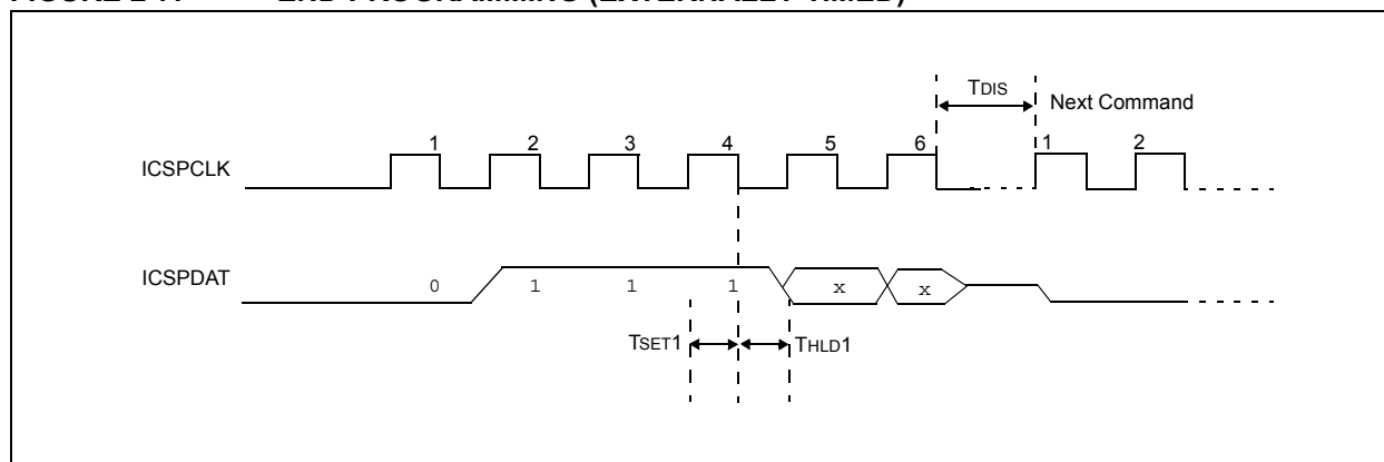
FIGURE 2-7: END PROGRAMMING (EXTERNALLY TIMED)
