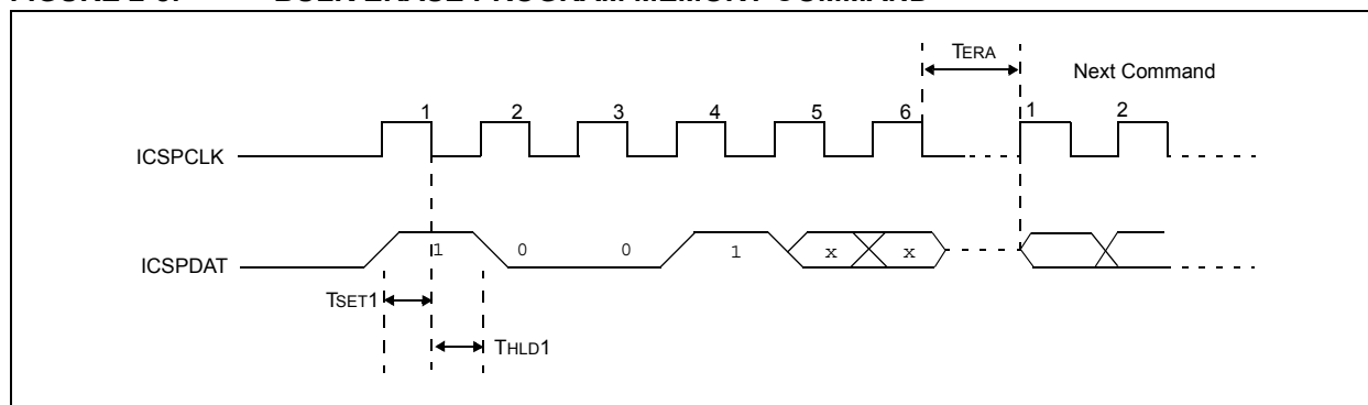
FIGURE 2-8: BULK ERASE PROGRAM MEMORY COMMAND
