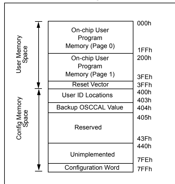
FIGURE 2-1: PIC16F506 PROGRAM MEMORY MAP
