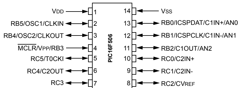
FIGURE 1-1: PIN DIAGRAMS
