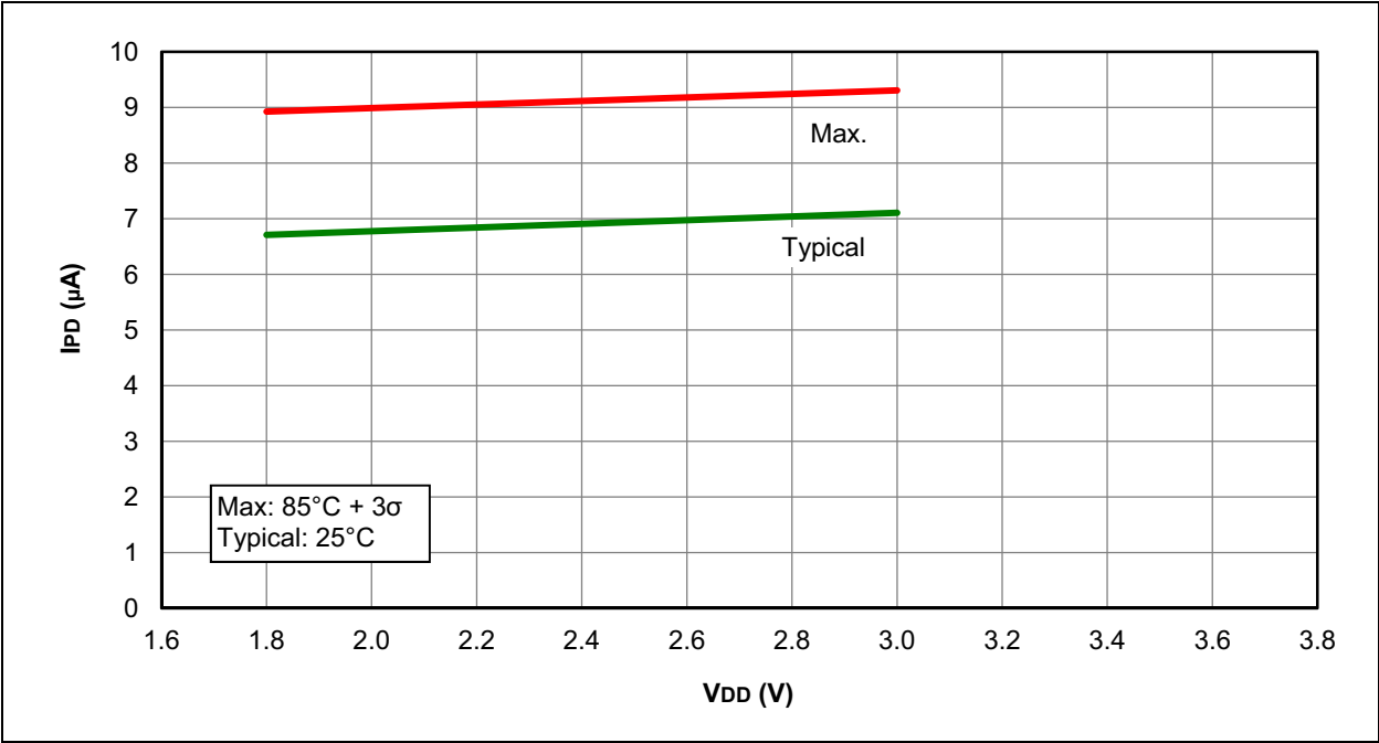
FIGURE 31-37: I_{PD} , COMPARATOR, LOW-POWER MODE ( C_{xSP} = 0 ), PIC16LF1825/1829 ONLY
