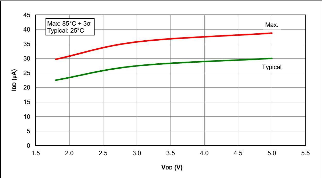
FIGURE 31-2: I_{DD} , LP OSCILLATOR MODE ( F_{osc} = 32\text{ kHz} ), PIC16F1825/1829 ONLY
