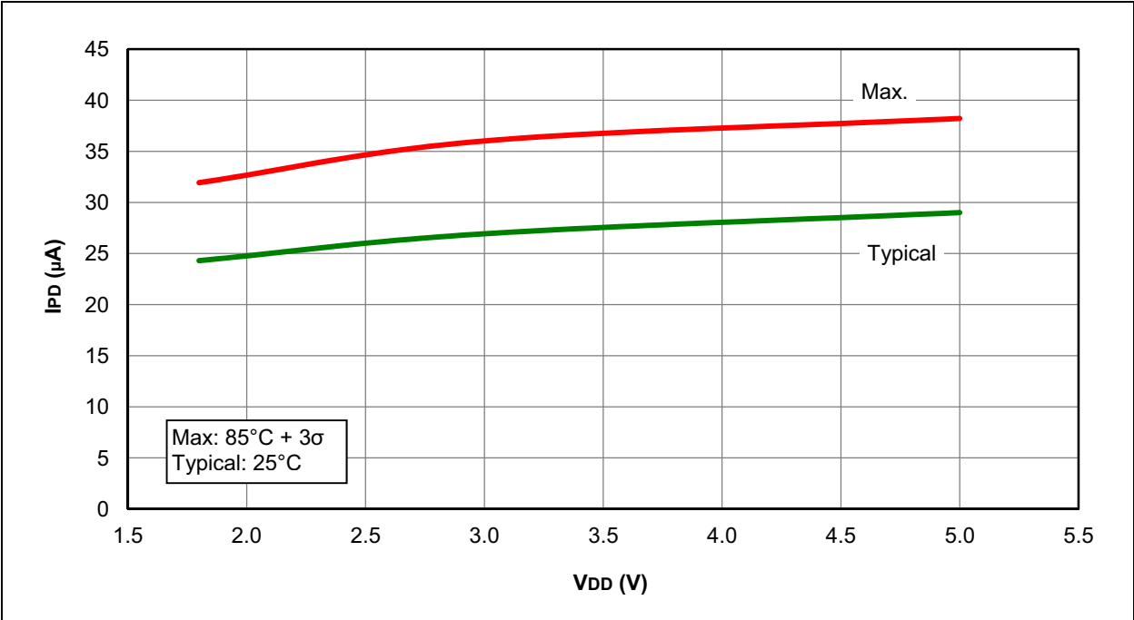
FIGURE 31-38: I_{PD} , COMPARATOR, LOW-POWER MODE ( C_{xSP} = 0 ), PIC16F1825/1829 ONLY
