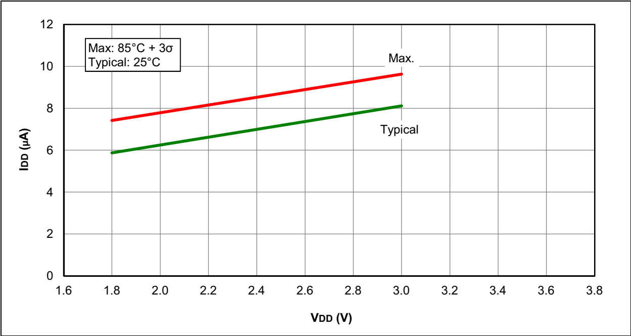
FIGURE 31-1: I_{DD} , LP OSCILLATOR MODE ( F_{osc} = 32\text{ kHz} ), PIC16LF1825/1829 ONLY
