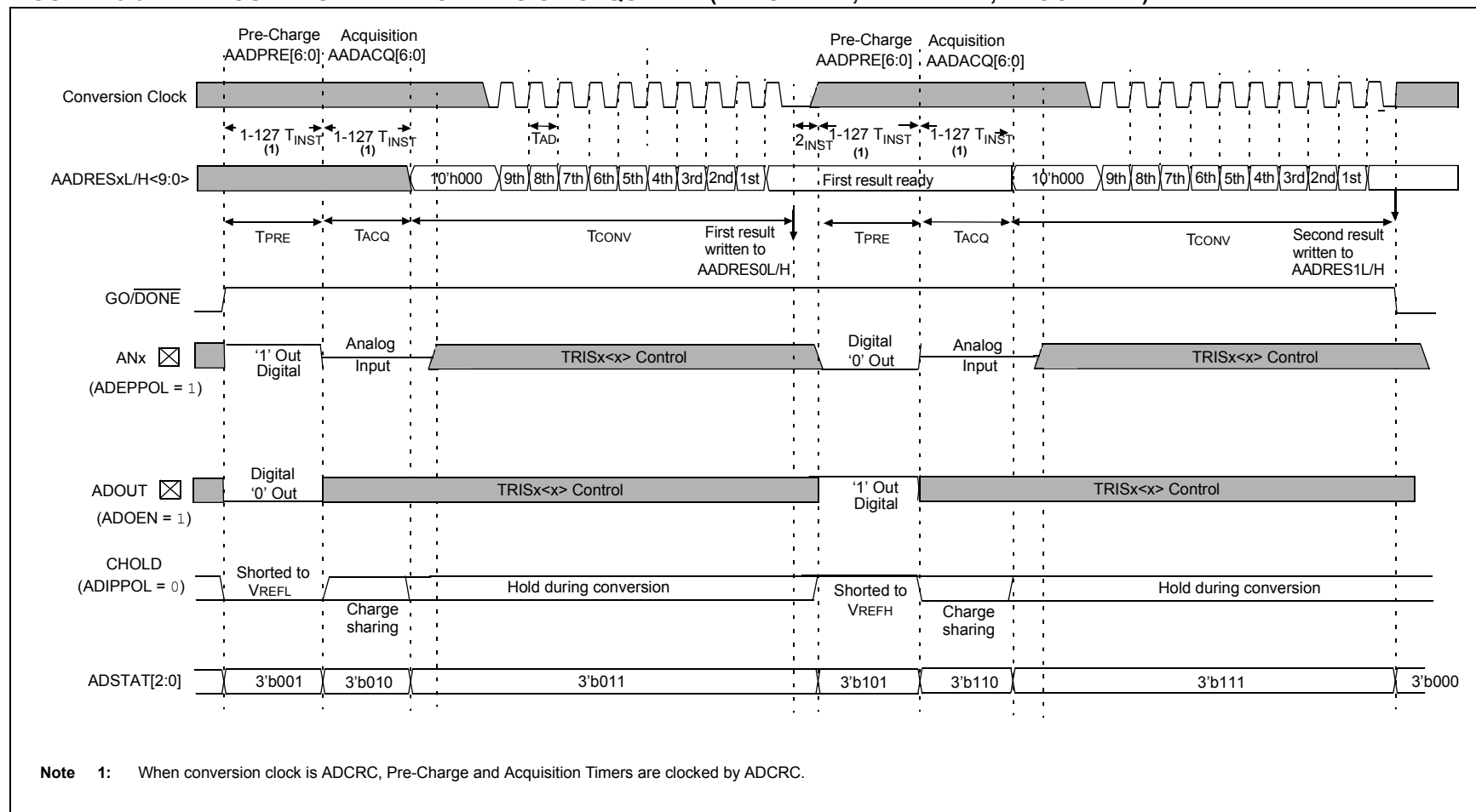
FIGURE 16-9: DOUBLE SAMPLE CONVERSION SEQUENCE (ADDSN = 1, ADIPEN = 1, ADOEN = 1)
