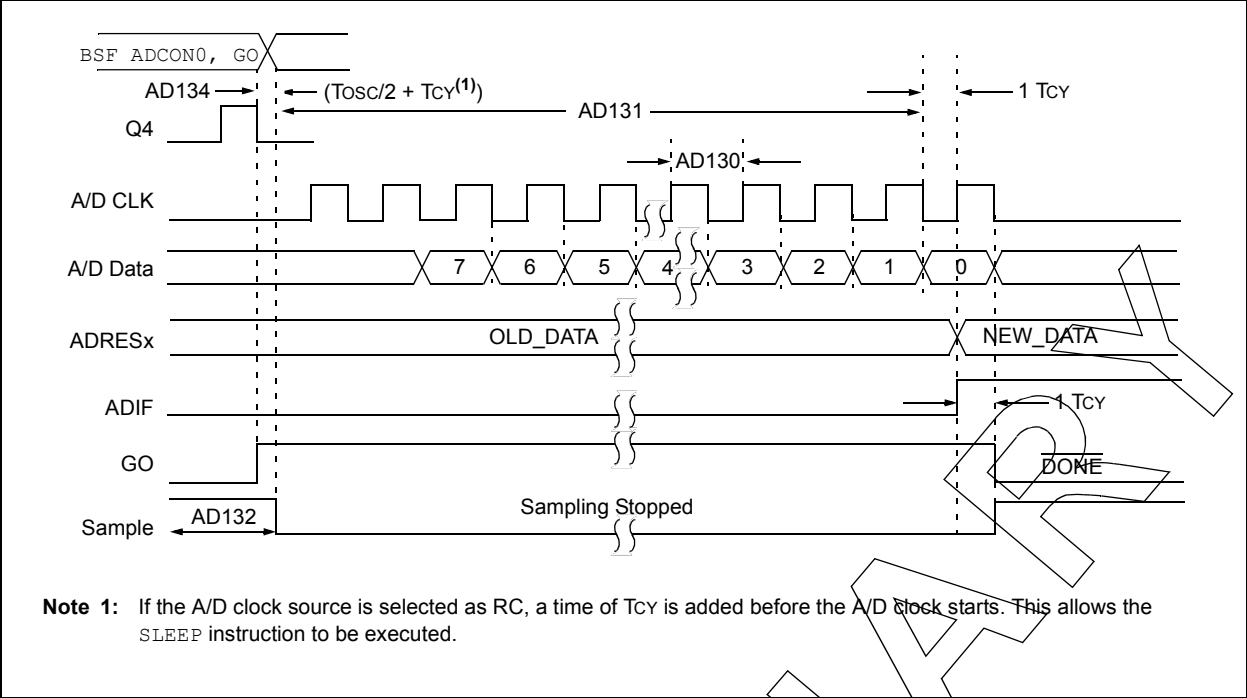
FIGURE 25-12: PIC16(L)F1512/3 A/D CONVERSION TIMING (SLEEP MODE)
