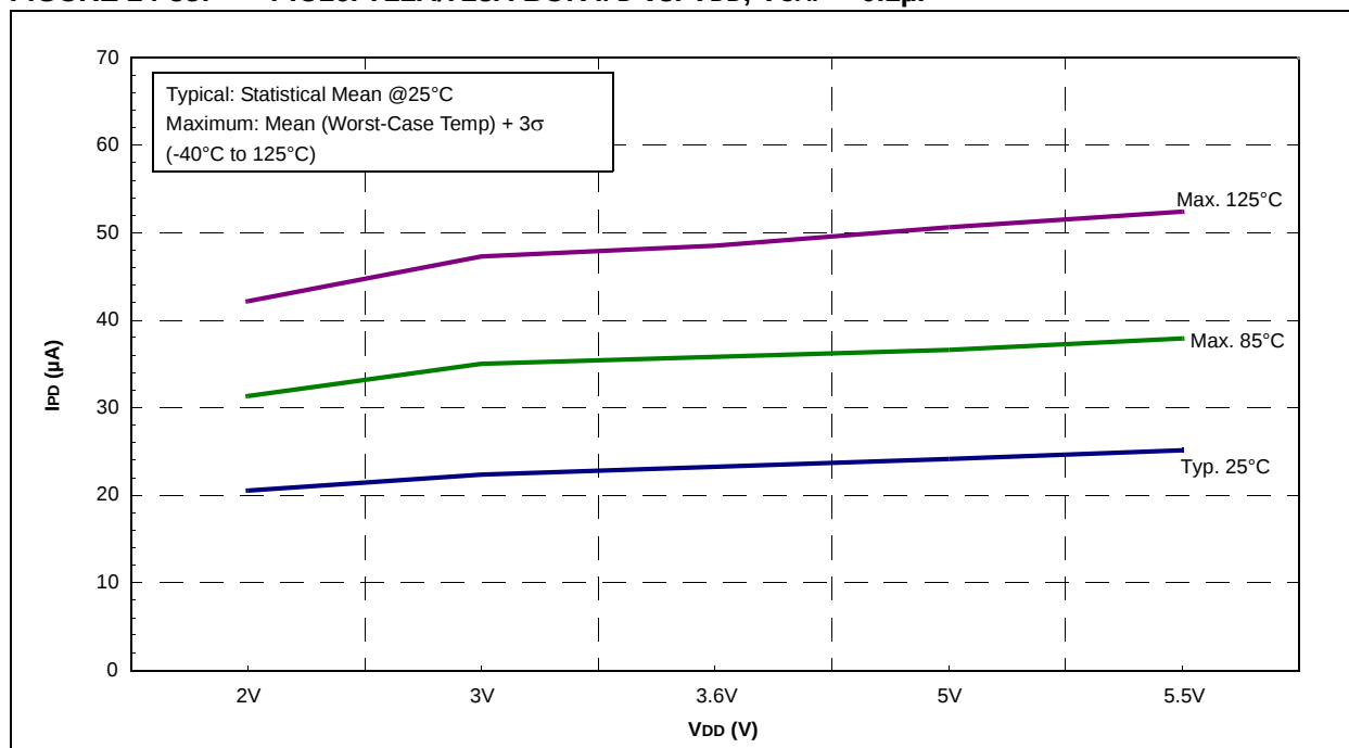
FIGURE 24-33: PIC16F722A/723A BOR I_{PD} vs. V_{DD} , V_{CAP} = 0.1\mu F
