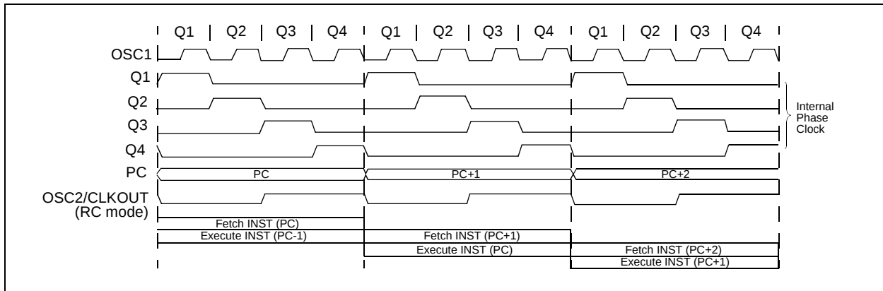
FIGURE 1-2: CLOCK/INSTRUCTION CYCLE
