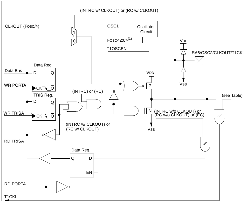
FIGURE 3-7: BLOCK DIAGRAM OF RA6/OSC2/CLKOUT/T1CKI PIN
