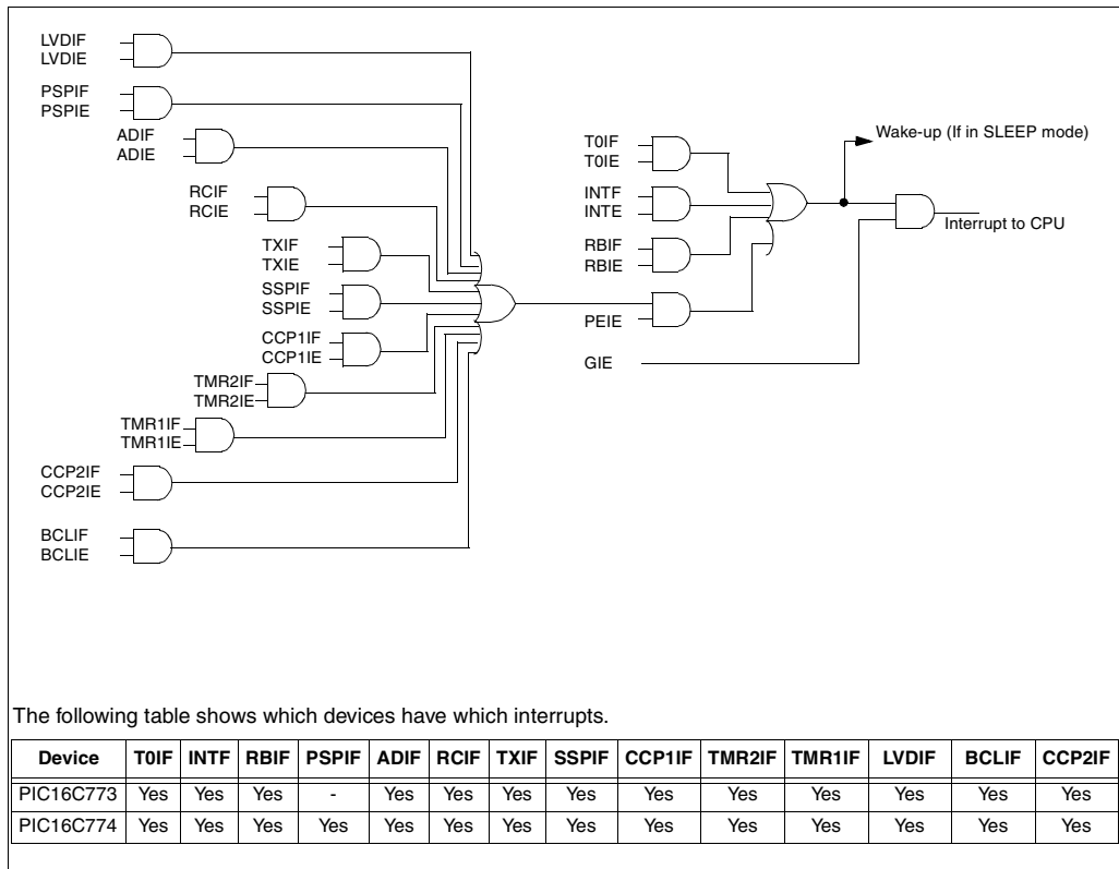
FIGURE 12-11: INTERRUPT LOGIC
