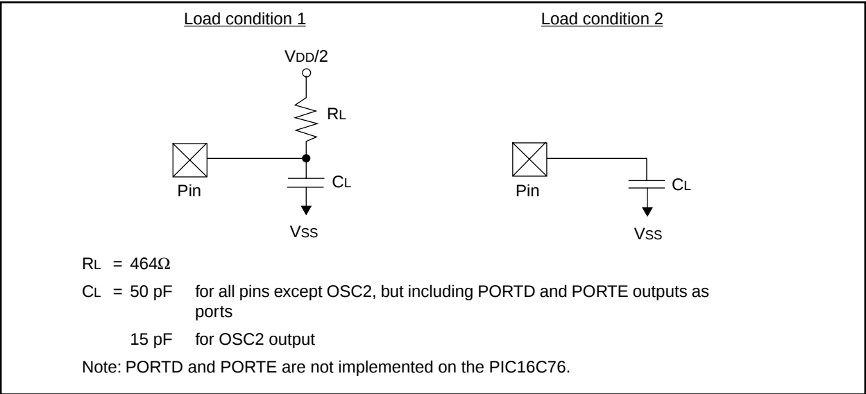
FIGURE 20-1: LOAD CONDITIONS
