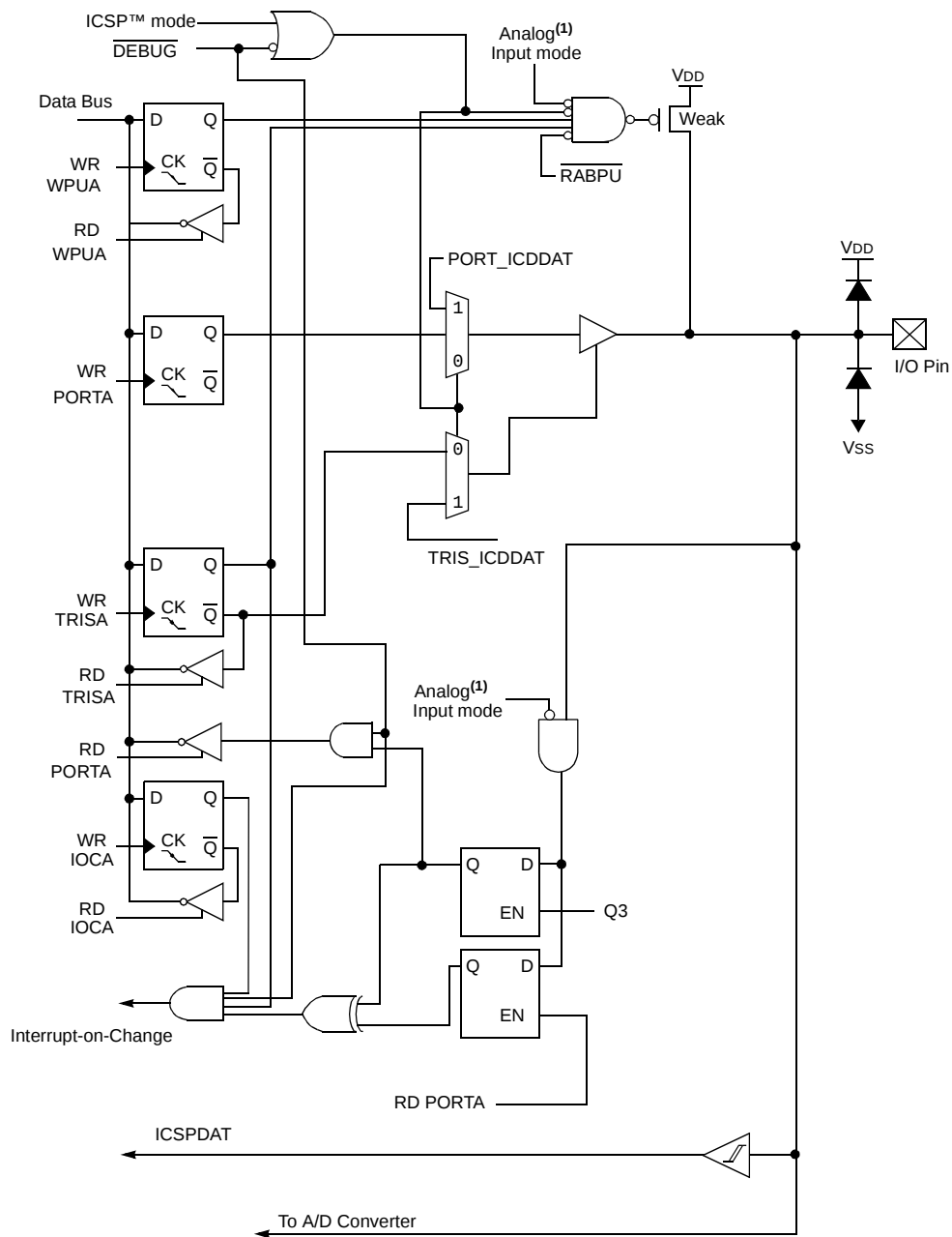
FIGURE 6-1: BLOCK DIAGRAM OF RA0
