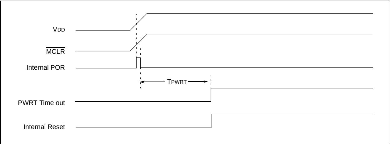
FIGURE 3-7: TIME-OUT SEQUENCE ON POWER-UP ( \overline{\text{MCLR}} WITH \text{V}_{\text{DD}} ): CASE 3
