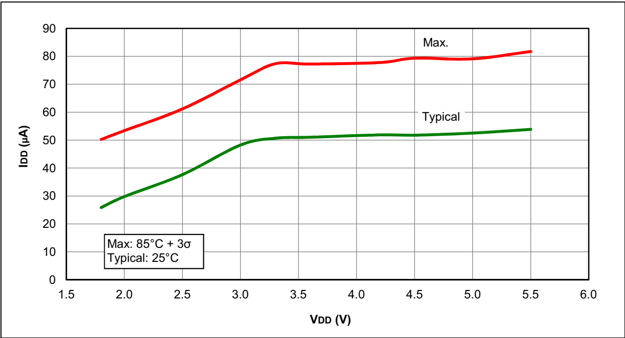
FIGURE 31-10: I_{DD} , EXTERNAL CLOCK (ECL), LOW-POWER MODE, F_{osc} = 500\text{ kHz} , PIC16F1938/9 ONLY
