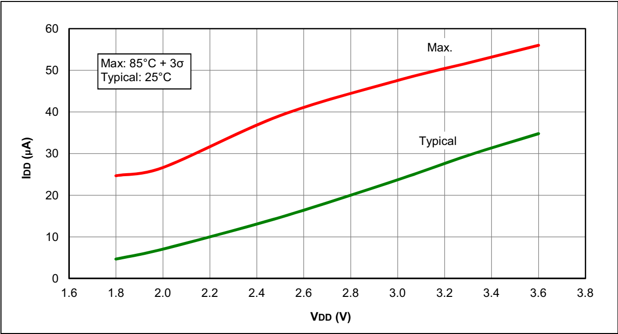
FIGURE 31-9: I_{DD} , EXTERNAL CLOCK (ECL), LOW-POWER MODE, F_{osc} = 500\text{ kHz} , PIC16LF1938/9 ONLY
