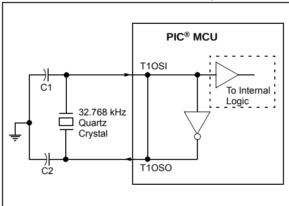
FIGURE 5-5: QUARTZ CRYSTAL OPERATION (TIMER1 OSCILLATOR)
