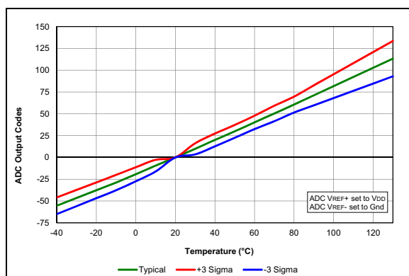
FIGURE 38-44: Temp. Indicator Slope Normalized to 20^\circ C , High Range, V_{DD} = 5.5V , PIC16F18854 Only.
