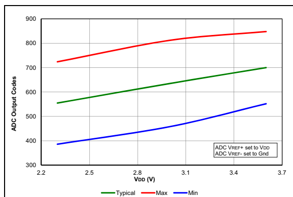
FIGURE 38-43: Temp. Indicator Initial Offset, Low Range, Temp. = 20^\circ C , PIC16LF18854 Only.
