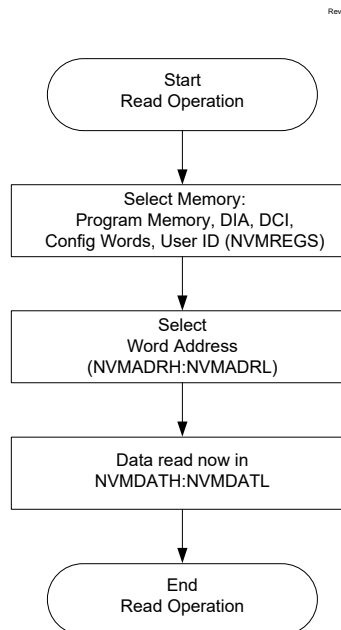
Figure 6-1. Flash Program Memory Read Flowchart
