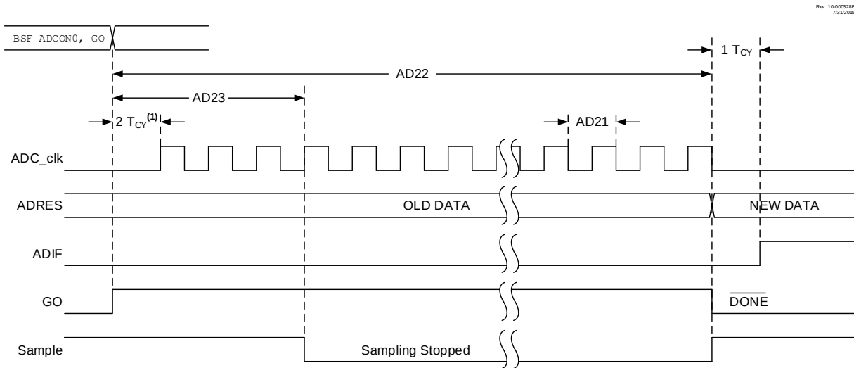
Figure 40-11. ADC Conversion Timing (ADC Clock from F_{RC} )
