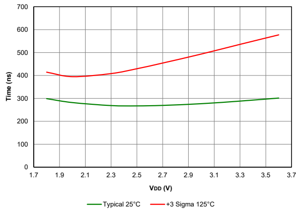
Figure 41-89. Band Gap Ready Time, PIC16LF18455/56 only
