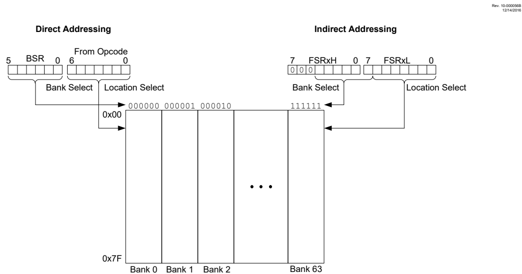
Figure 5-9. Traditional/Banked Data Memory Map
