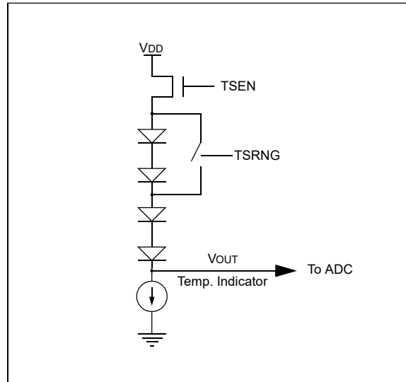
Figure 31-1. Temperature Circuit Block Diagram
