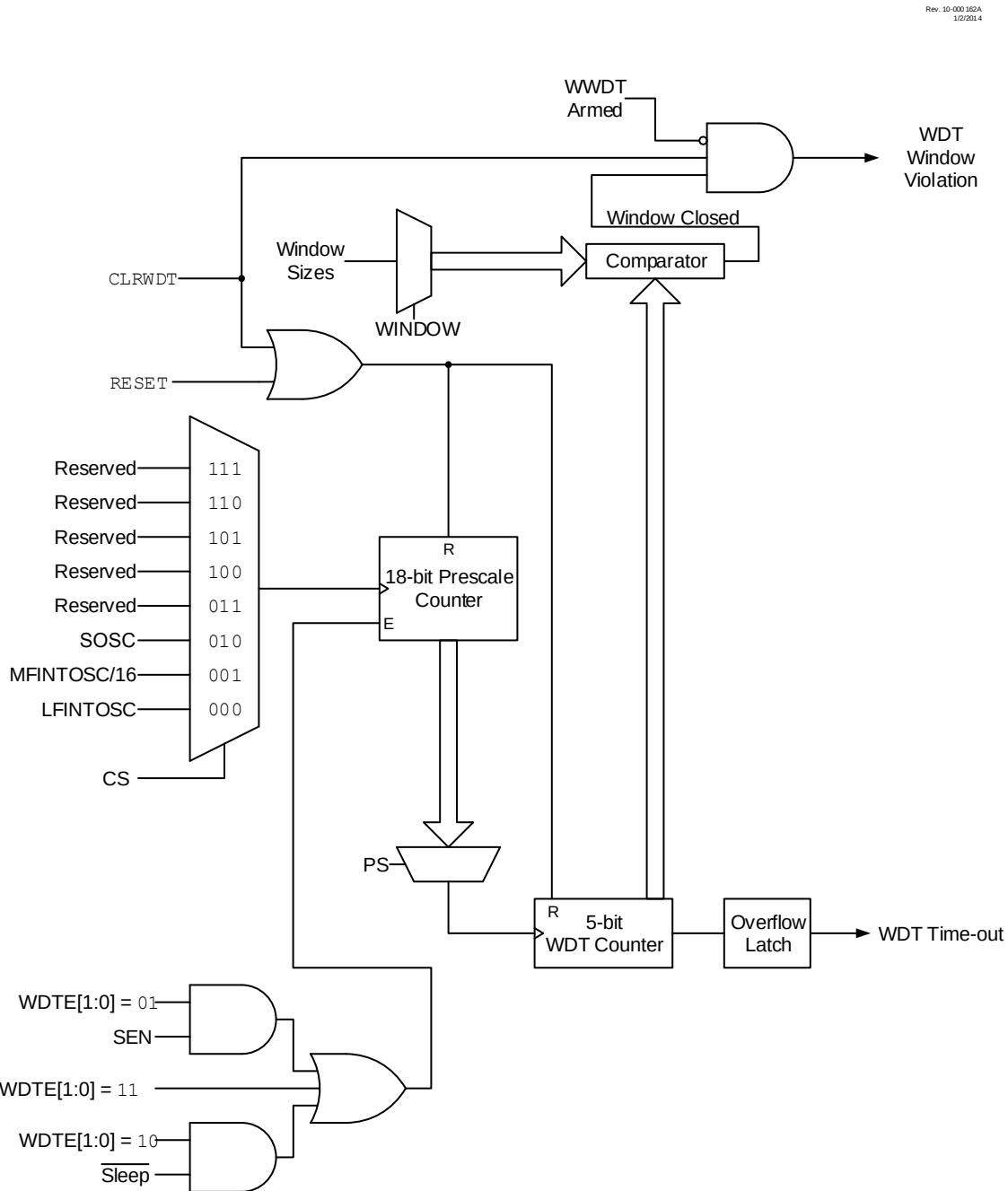
Figure 11-1. Windowed Watchdog Timer Block Diagram
