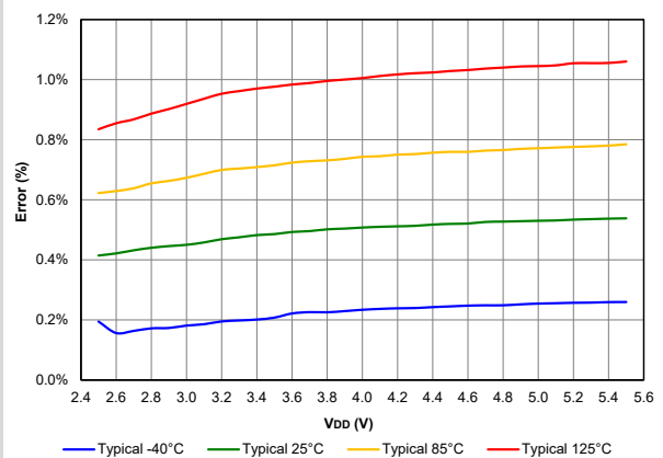
Figure 41-92. FVR Voltage Error 1x, PIC16F18455/56 only
