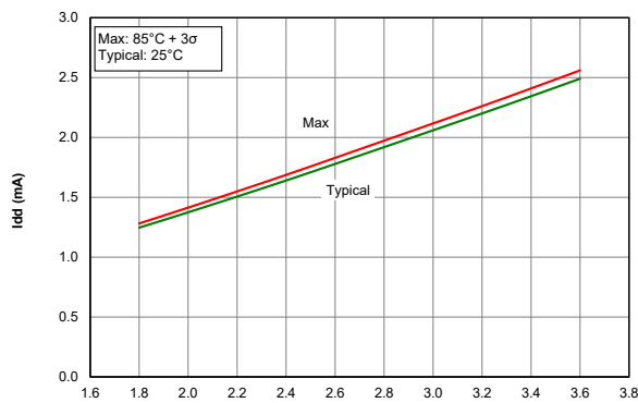
Figure 41-19. I_{DD} HFINTOSC Mode, F_{OSC} = 16 MHz, PIC16LF18455/56 only
