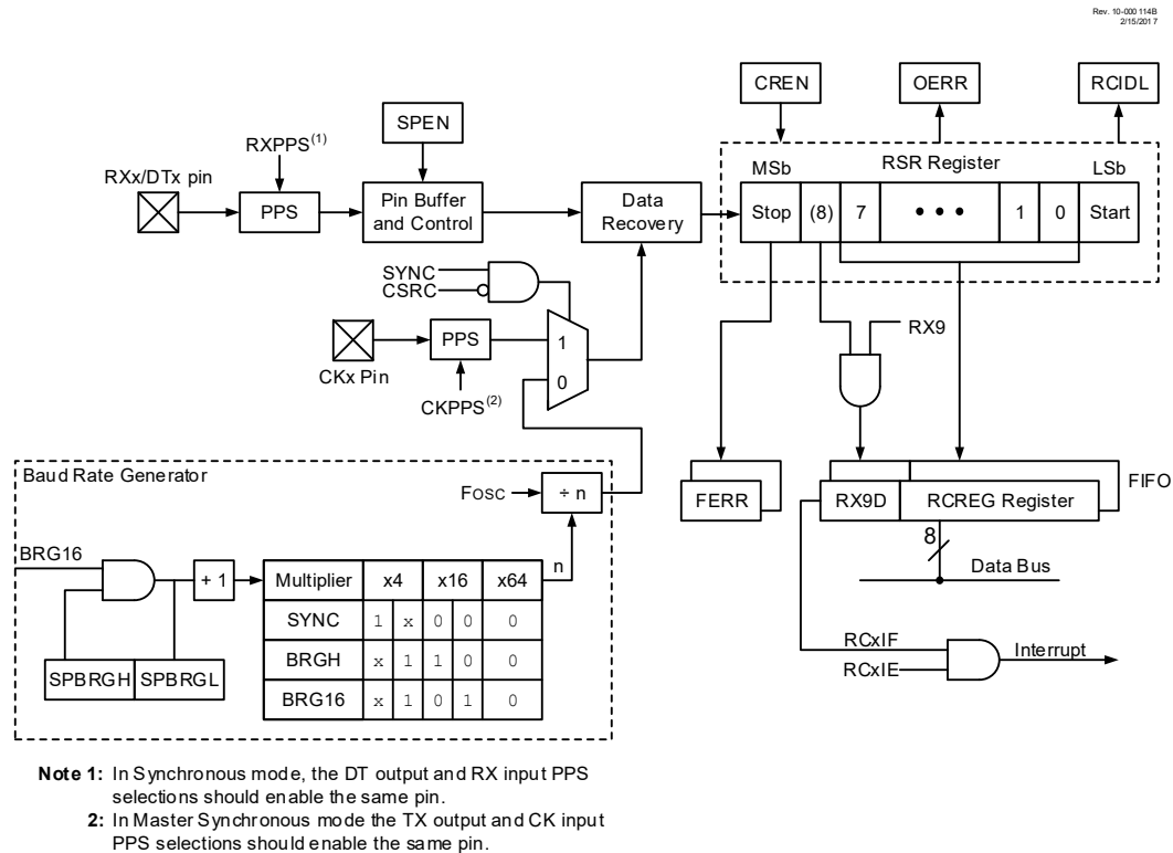
Figure 28-2. EUSART Receive Block Diagram
