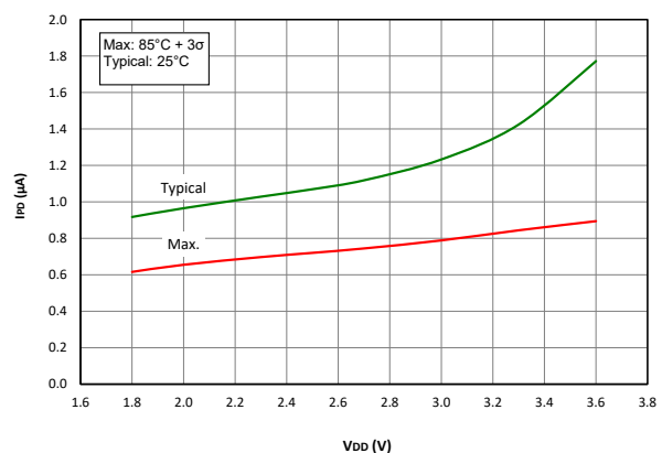
Figure 41-2. I_{PD} Watchdog Timer (WDT) PIC16LF18455/56 only
