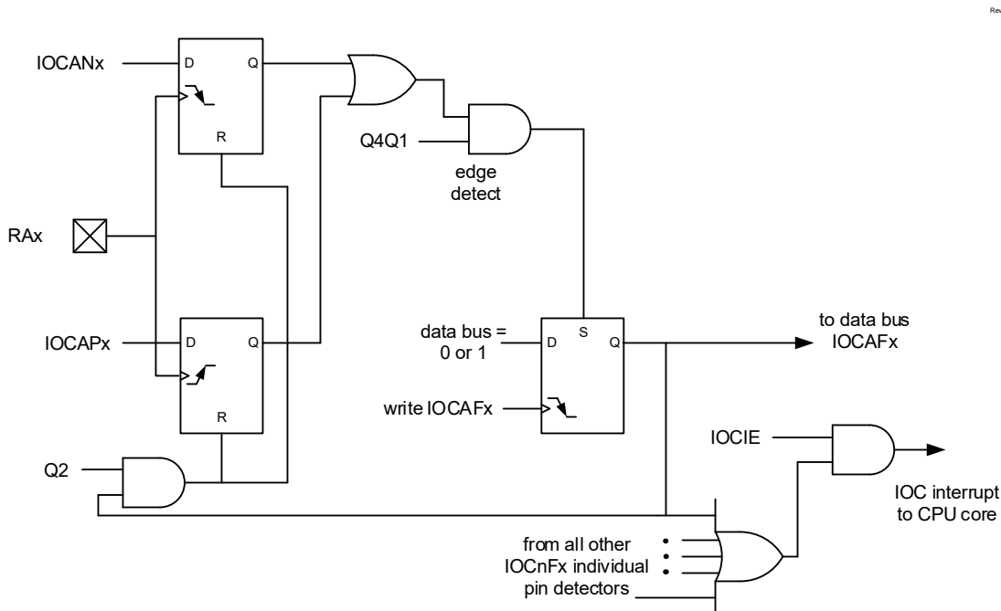
Figure 15-1. Interrupt-on-Change Block Diagram (PORTA Example)
