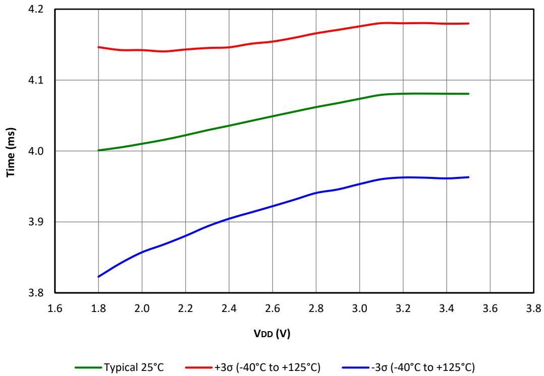
Figure 41-115. WDT Time-Out Period, PIC16LF18455/56 only
