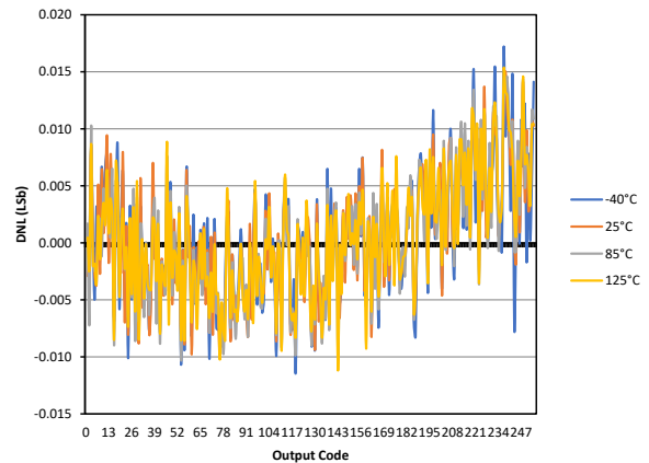
Figure 41-70. Typical DAC INL Error, V_{DD} = 5.0V , V_{REF} = \text{External } 5V , PIC16F18455/56 only
