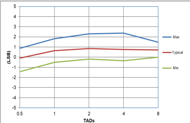
Figure 41-64. ADC 12-Bit Mode, Single-Ended Gain Error, V_{DD} = 3.0V , V_{REF} = 3.0V , -40^{\circ}C to 85^{\circ}C , All devices
