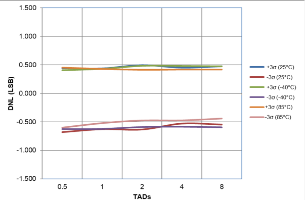
Figure 41-54. ADC 12-Bit Mode, Single-Ended DNL, V_{DD} = 3.0V , V_{REF} = 3.0V , All devices
