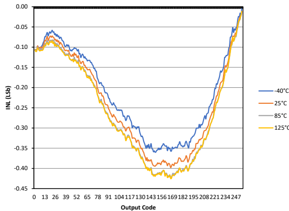
Figure 41-69. Typical DAC INL Error, V_{DD} = 3.0V , V_{REF} = \text{External } 3V , All devices
