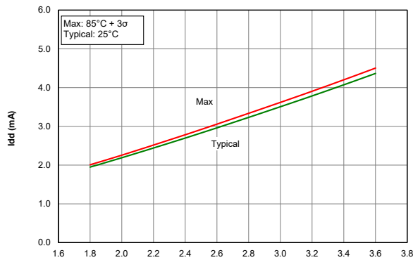
Figure 41-15. I_{DD} HS Oscillator 32 MHz, PIC16LF18455/56 only
