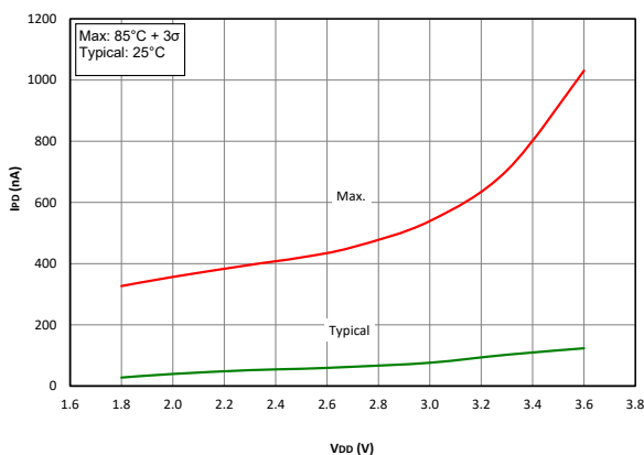
Figure 41-1. I_{PD} Base, Low-Power Sleep Mode PIC16LF18455/56 only
