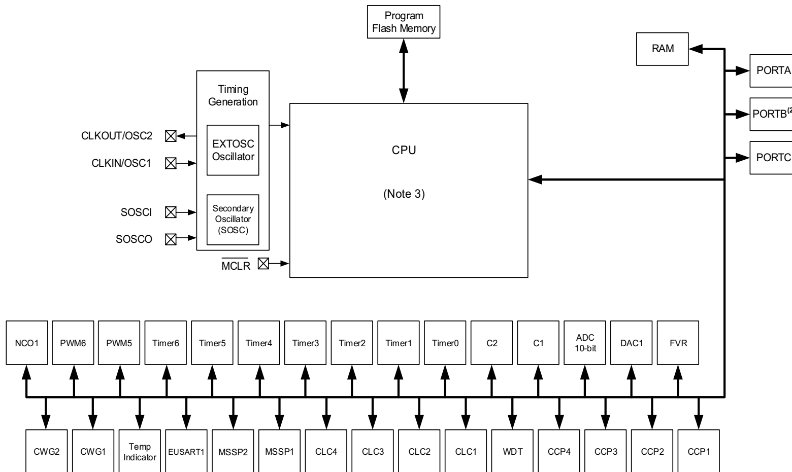
FIGURE 1-1: PIC16(L)F18325/18345 BLOCK DIAGRAM
