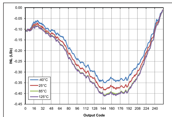
FIGURE 36-72: Typical DAC INL Error, V_{DD} = 5.0\text{V} , V_{REF} = \text{External } 5\text{V} , PIC16F18325/18345 Only
