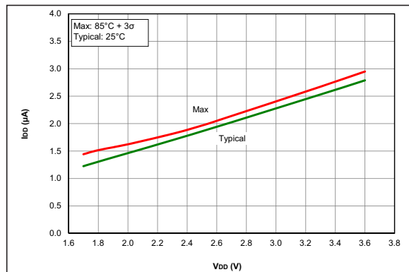
FIGURE 36-3: I_{DD} , HS Oscillator, 32 MHz, PIC16LF18325/18345 Only
