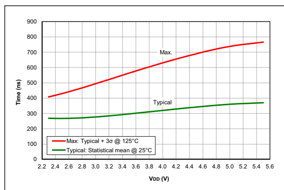
FIGURE 36-89: Comparator Response Time Rising edge, PIC16F18325/18345 Only
