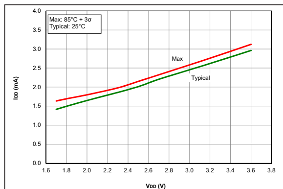
FIGURE 36-5: I_{DD} , HFINTOSC Mode, F_{OSC} = 32 MHz, PIC16LF18325/18345 Only
