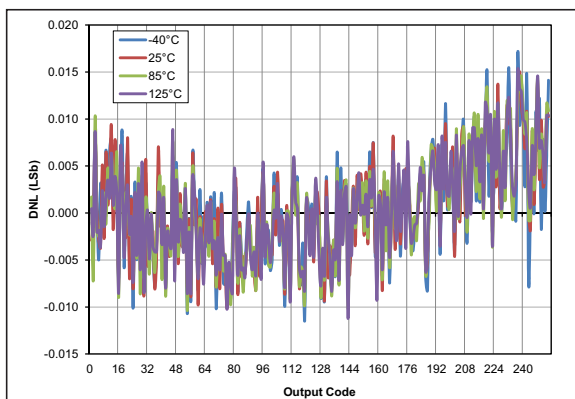
FIGURE 36-71: Typical DAC DNL Error, V_{DD} = 5.0\text{V} , V_{REF} = \text{External } 5\text{V} , PIC16F18325/18345 Only
