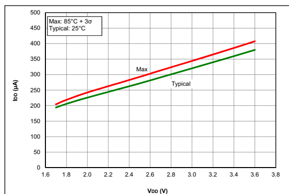
FIGURE 36-1: I_{DD} , XT Oscillator, 4 MHz, PIC16LF18325/18345 Only
