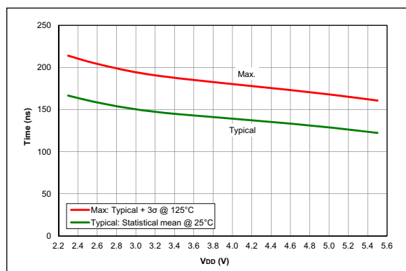
FIGURE 36-87: Comparator Response Time Falling edge, PIC16F18325/18345 Only
