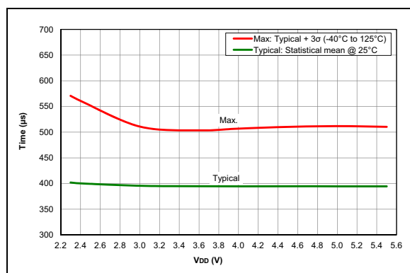
FIGURE 36-113: Wake From Sleep, VREGPM = 1, LFINTOSC, PIC16F18324/18344 Only
