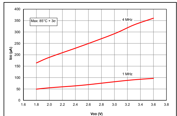
FIGURE 31-12: I_{DD} Maximum, EC Oscillator MP Mode, PIC16LF1782/3 Only.
