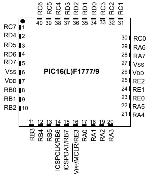
FIGURE 5: 40-PIN VQFN (5x5x0.9 mm)
