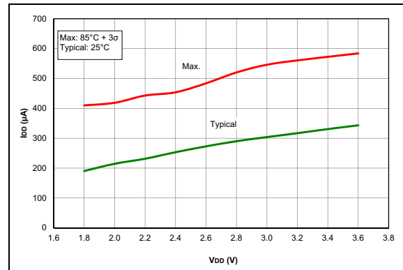
FIGURE 38-46: I_D , Op Amp, NP Mode ( V_{REFPM} = 0 ), PIC16LF1777/8/9 Only.
