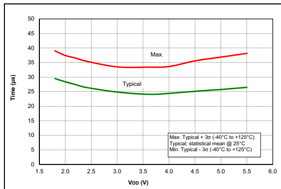
FIGURE 38-76: Wake From Sleep, V_{REGPM} = 1 .
