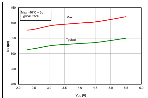
FIGURE 38-51: I_{D} , Comparator, NP Mode ( V_{REGPM} = 0 ), PIC16F1777/8/9 Only.
