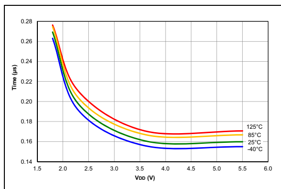
FIGURE 38-133: COG Dead-Band Delay, DBR/DBF = 32, Typical Measured Values.
