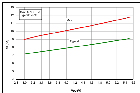
FIGURE 38-41: I_{DD} , Brown-Out Reset (BOR), BORV = 1 , PIC16F1777/8/9 Only.
