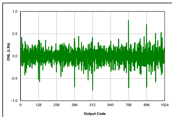
FIGURE 38-78: ADC 10-bit Mode, Single-Ended DNL, V_{DD} = 3.0V , T_{AD} = 1\text{ }\mu\text{s} , 25^\circ\text{C} .
