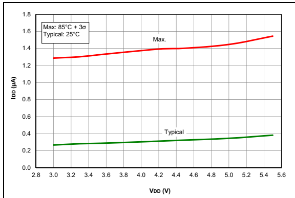
FIGURE 38-43: I_D , LP Brown-Out Reset (LPBOR = 0), PIC16F1777/8/9 Only.
