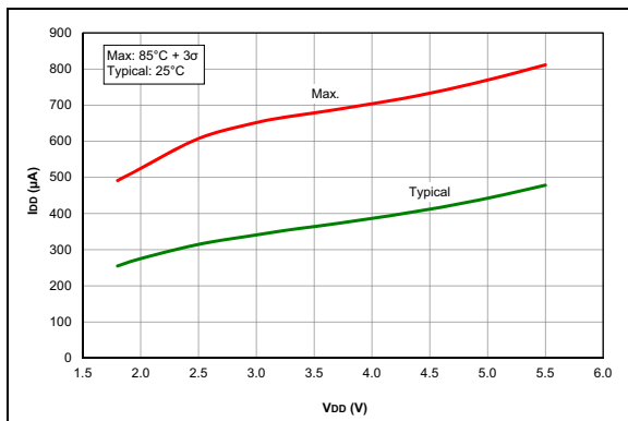
FIGURE 38-47: I_D , Op Amp, NP Mode ( V_{REFPM} = 0 ), PIC16F1777/8/9 Only.
