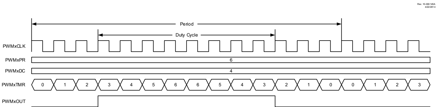
FIGURE 26-7: CENTER ALIGNED PWM MODE TIMING DIAGRAM
