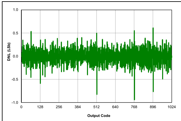
FIGURE 38-79: ADC 10-bit Mode, Single-Ended DNL, V_{DD} = 3.0V , T_{AD} = 4\text{ }\mu\text{S} , 25^\circ\text{C} .
