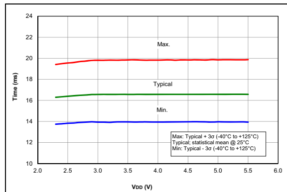
FIGURE 38-60: WDT Time-Out Period, PIC16F1777/8/9 Only.
