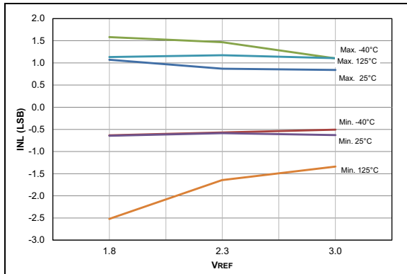
FIGURE 38-85: ADC 10-bit Mode, Single-Ended INL, V_{DD} = 3.0V , T_{AD} = 1\text{ }\mu\text{S} .
