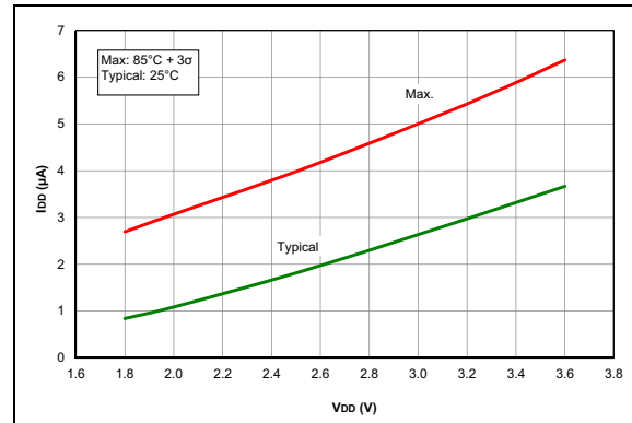
FIGURE 38-44: I_D , Timer1 Oscillator, F_{OSC} = 32\text{ kHz} , PIC16LF1777/8/9 Only.
