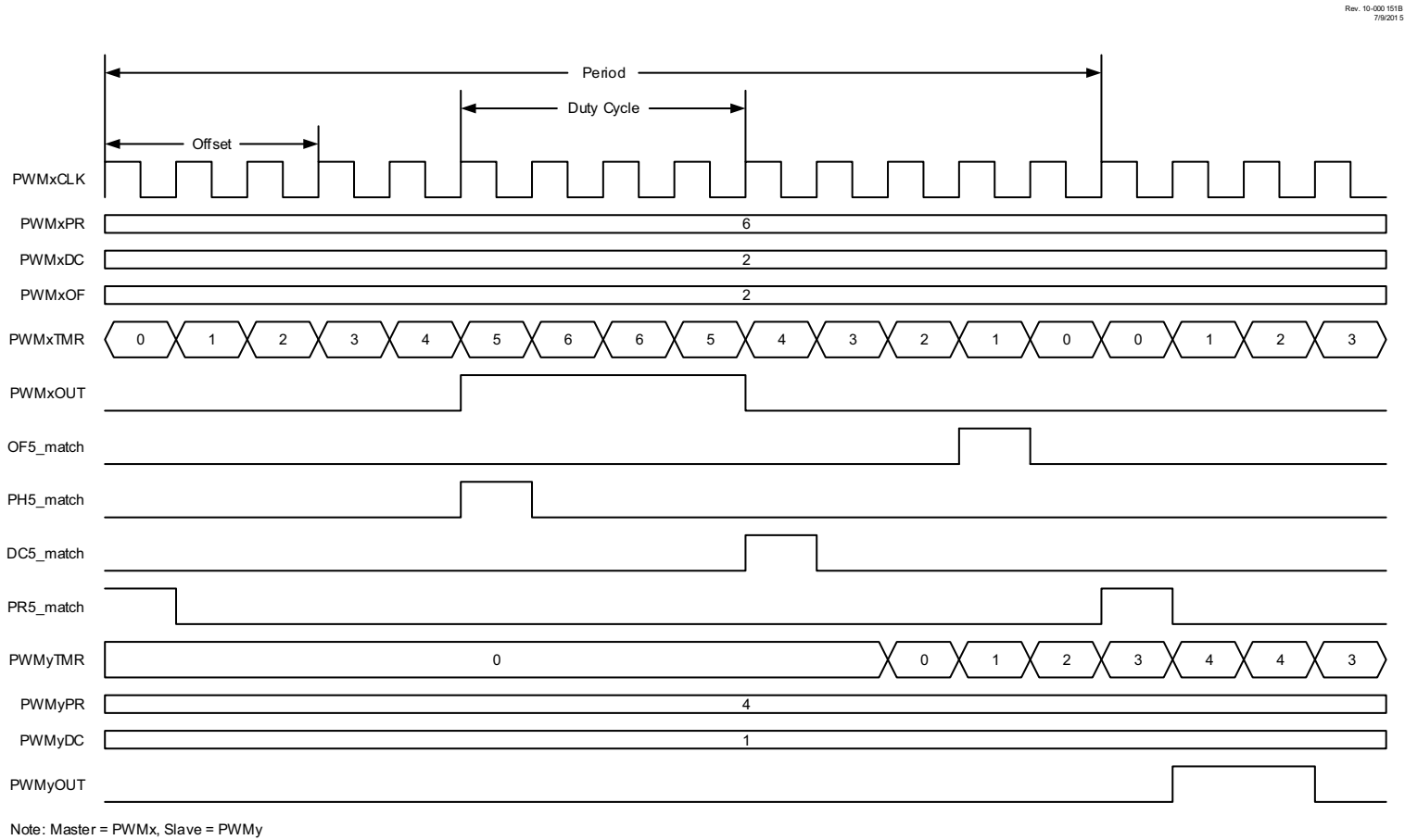
FIGURE 26-13: OFFSET MATCH ON DECREMENTING TIMER TIMING DIAGRAM
