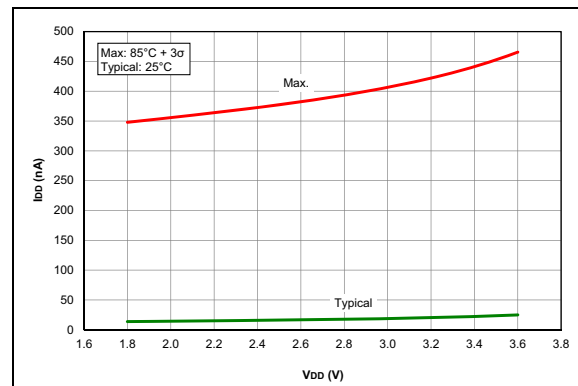
FIGURE 38-48: I_D , ADC Non-Converting, PIC16LF1777/8/9 Only.
