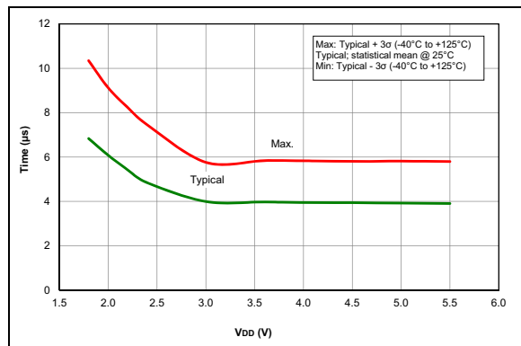
FIGURE 38-75: Wake From Sleep, V_{REGPM} = 0 .
