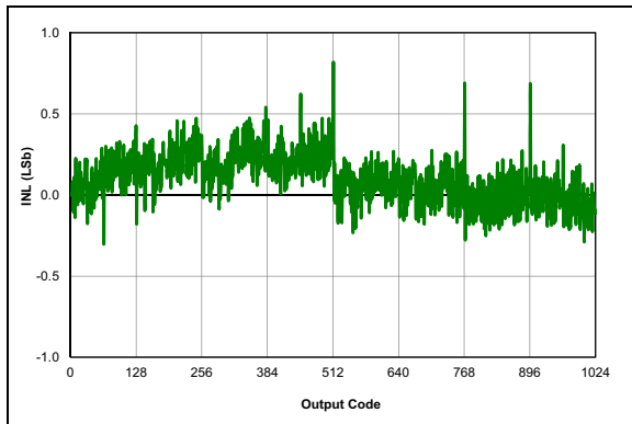
FIGURE 38-81: ADC 10-bit Mode, Single-Ended INL, V_{DD} = 3.0V , T_{AD} = 4\text{ }\mu\text{S} , 25^\circ\text{C} .
