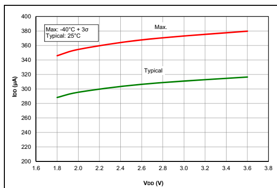
FIGURE 38-50: I_{D} , Comparator, NP Mode ( V_{REGPM} = 0 ), PIC16LF1777/8/9 Only.
