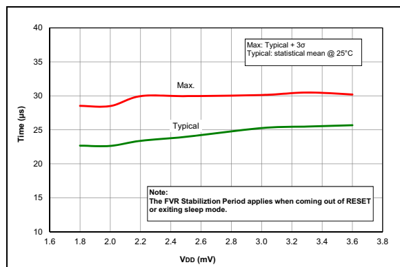
FIGURE 38-77: FVR Stabilization Period, PIC16LF1777/8/9 Only.
