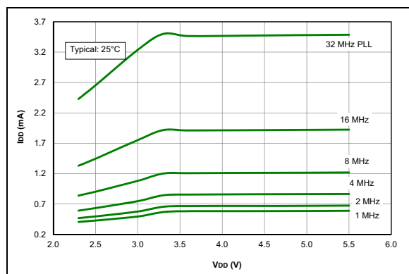
FIGURE 38-25: I_{DD} Typical, HFINTOSC Mode, PIC16F1777/8/9 Only.
