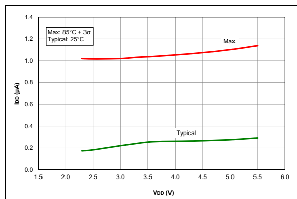
FIGURE 38-49: I_{D} , ADC Non-Converting, PIC16F1777/8/9 Only.
