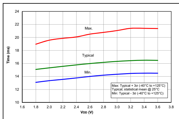
FIGURE 38-61: WDT Time-Out Period, PIC16LF1777/8/9 Only.
