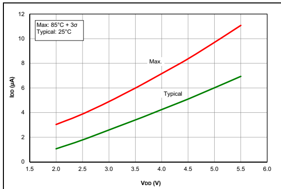
FIGURE 38-45: I_D , Timer1 Oscillator, F_{OSC} = 32\text{ kHz} , PIC16F1777/8/9 Only.
