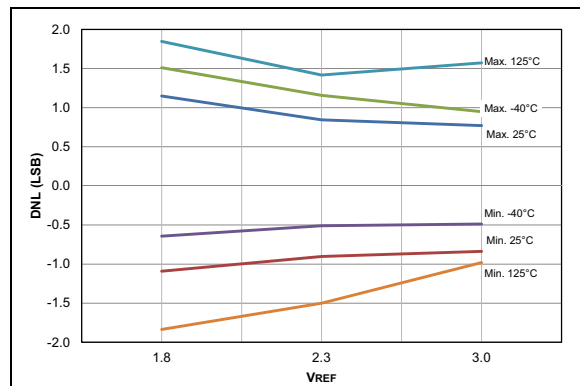
FIGURE 38-84: ADC 10-bit Mode, Single-Ended DNL, V_{DD} = 3.0V , T_{AD} = 1\text{ }\mu\text{S} .
