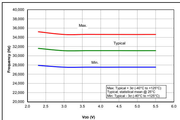
FIGURE 38-59: LFINTOSC Frequency, PIC16F1777/8/9 Only.
