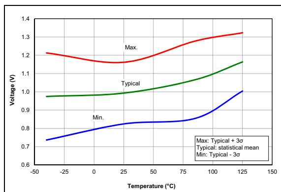
FIGURE 38-74: POR Rearm Voltage, NP Mode, PIC16LF1777/8/9 Only.
