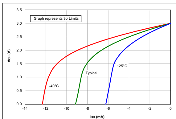
FIGURE 38-54: V_{OL} vs. I_{OH} Over Temperature, V_{DD} = 3.0V .
