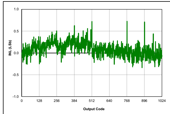
FIGURE 38-80: ADC 10-bit Mode, Single-Ended INL, V_{DD} = 3.0V , T_{AD} = 1\text{ }\mu\text{S} , 25^\circ\text{C} .
