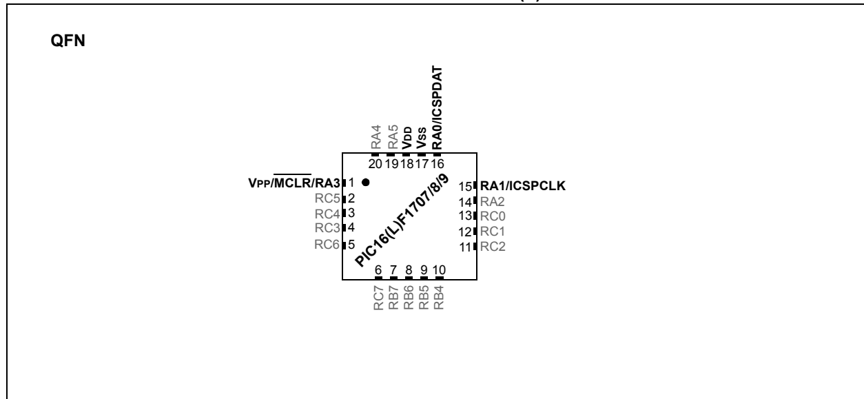
FIGURE 2-4: 20-PIN PACKAGE DIAGRAM FOR PIC16(L)F1707/8/9
