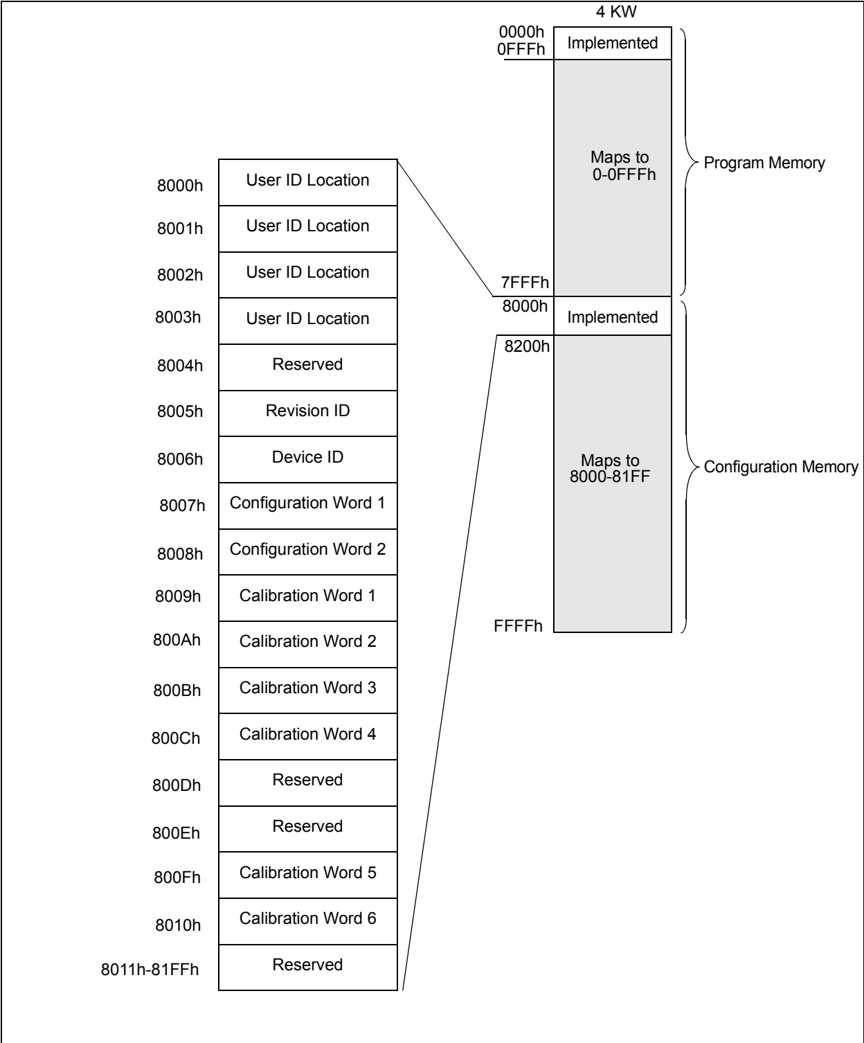
FIGURE 3-2: PIC16(L)F1704/8 PROGRAM MEMORY MAPPING
