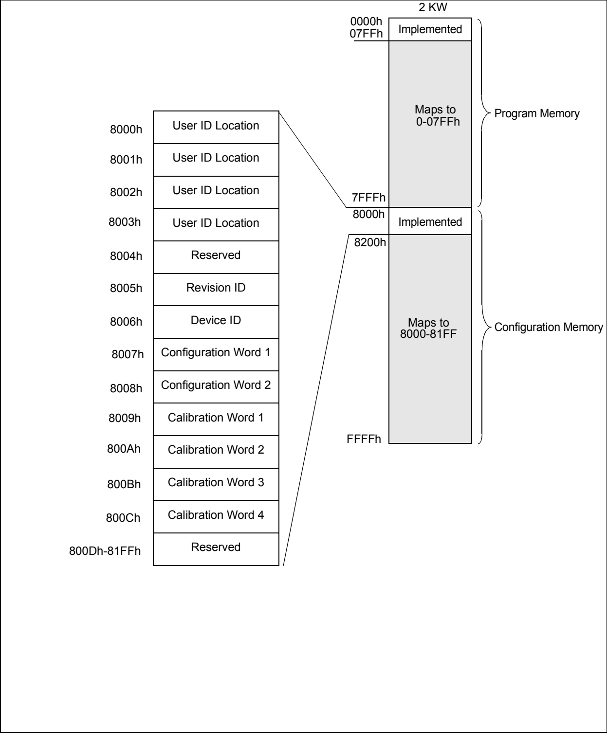
FIGURE 3-1: PIC16(L)F1703/7 PROGRAM MEMORY MAPPING
