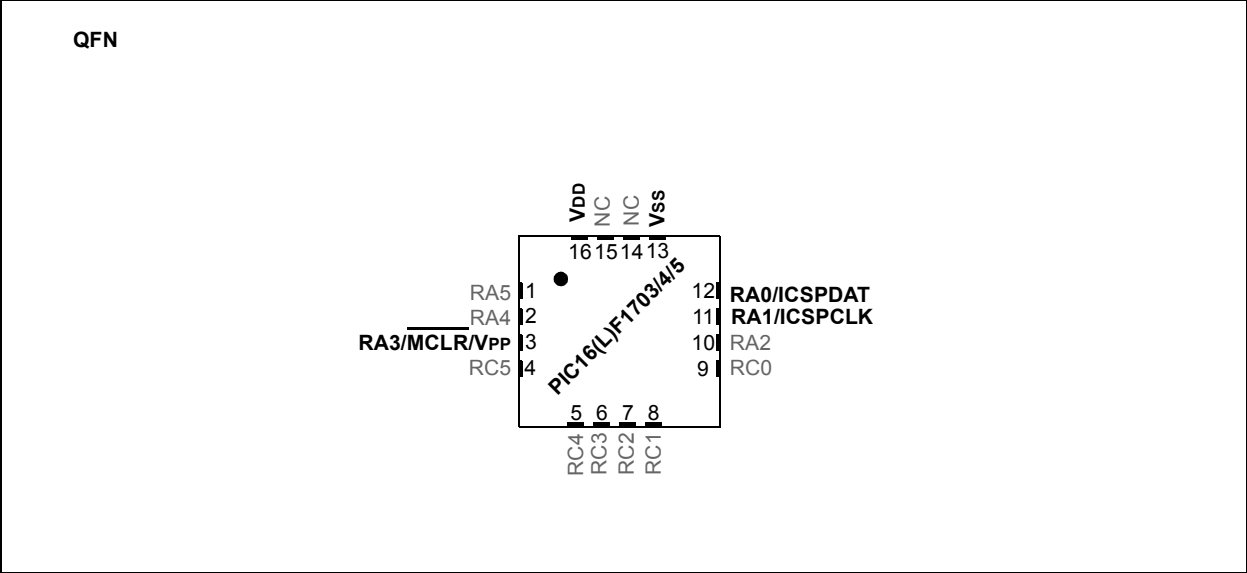
FIGURE 2-2: 16-PIN PACKAGE DIAGRAM FOR PIC16(L)F1703/4/5
