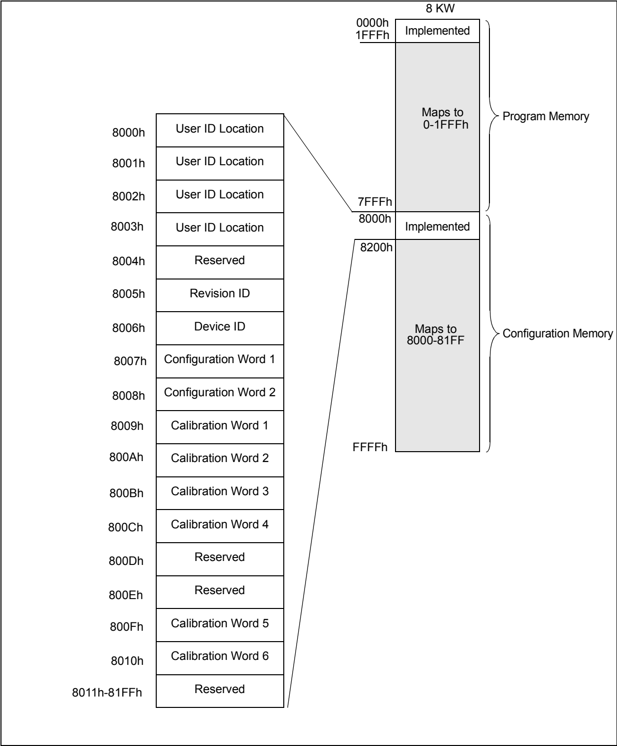
FIGURE 3-3: PIC16(L)F1705/9 PROGRAM MEMORY MAPPING
