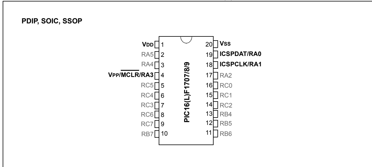
FIGURE 2-3: 20-PIN PACKAGE DIAGRAM FOR PIC16(L)F1707/8/9
