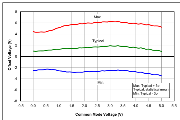
FIGURE 33-97: Op Amp, Offset over Common Mode Voltage, V_{DD} = 5.0V , T_{mp} = 25^\circ C PIC16F1704/8 Only.
