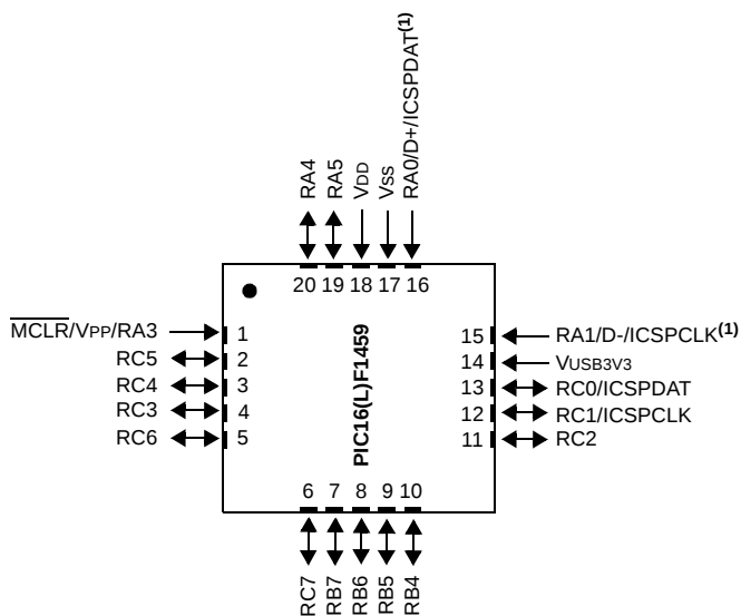
FIGURE 4: 20-PIN QFN DIAGRAM FOR PIC16(L)F1459
