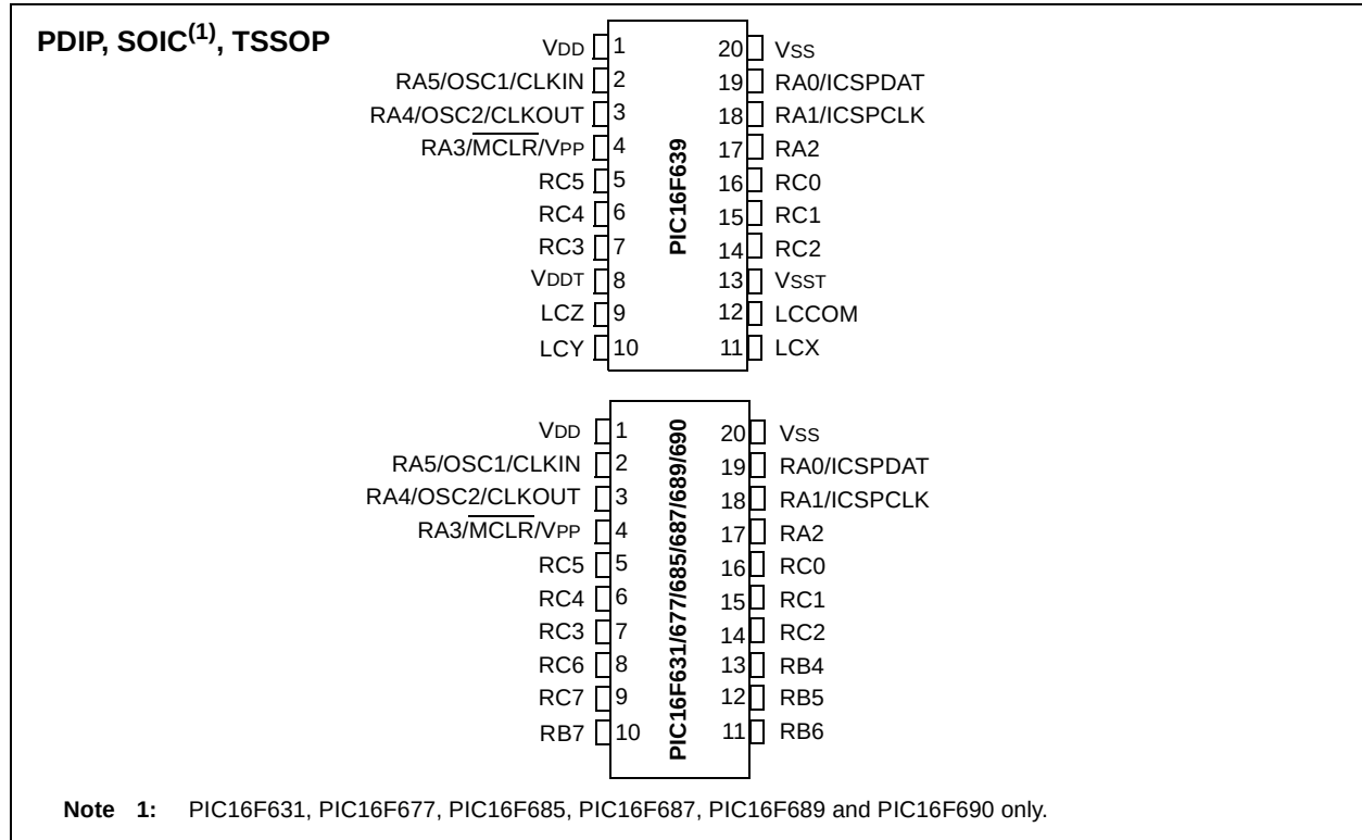
FIGURE 1-4: 20-PIN DIAGRAMS
