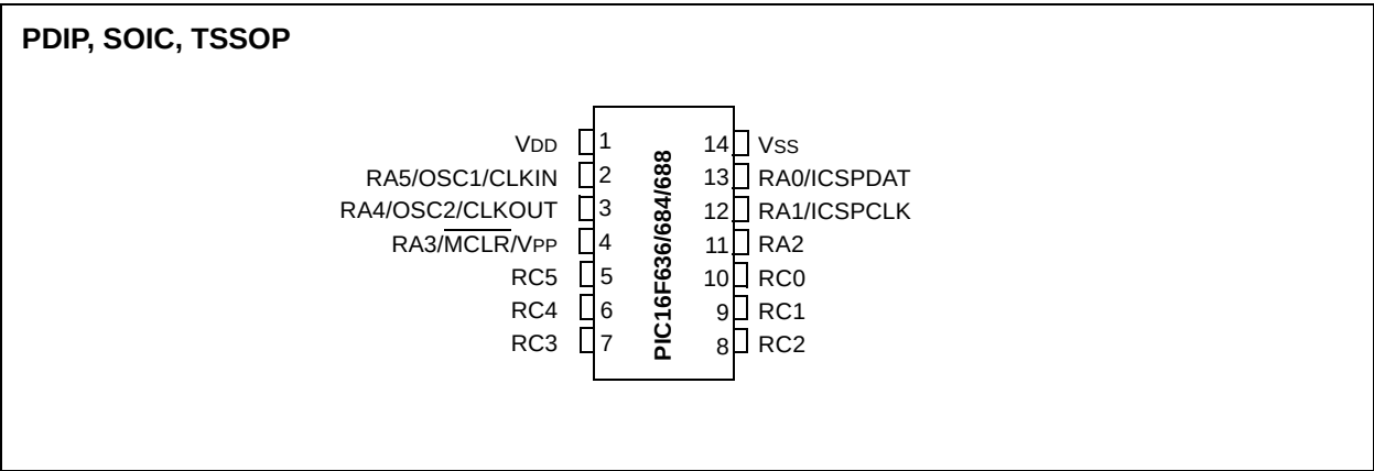
FIGURE 1-2: 14-PIN DIAGRAM FOR PIC16F636/684/688
