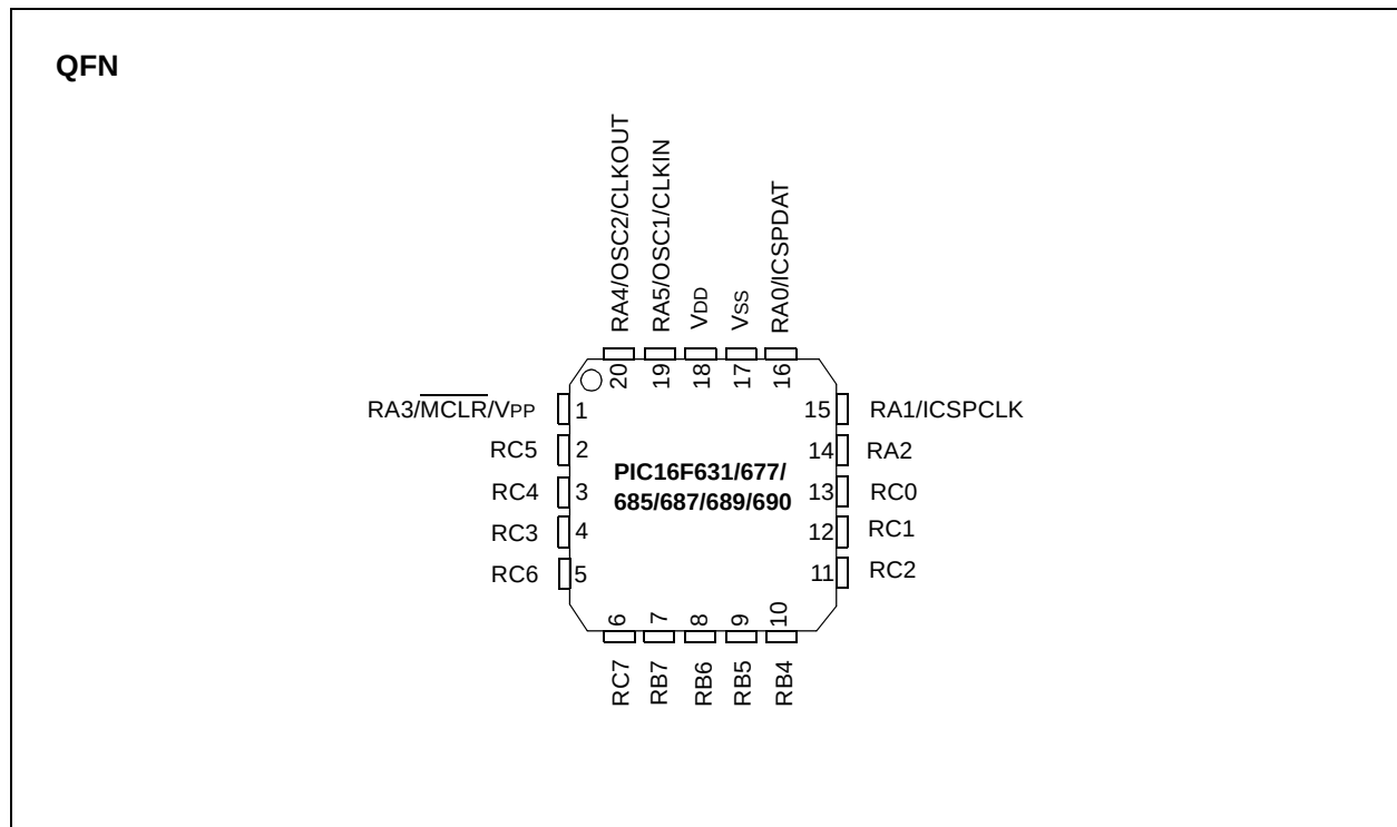
FIGURE 1-5: 20-PIN DIAGRAM FOR PIC16F631/677/685/687/689/690
