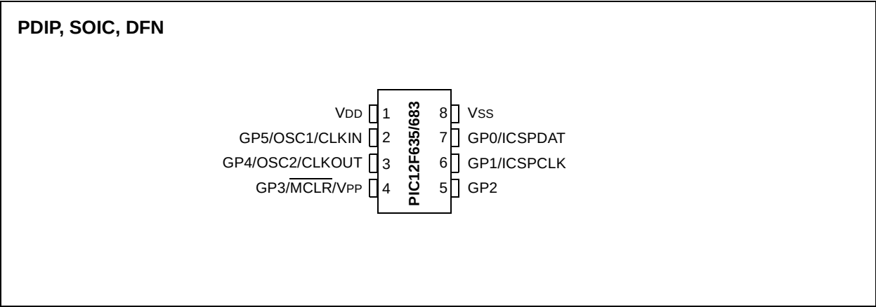
FIGURE 1-1: 8-PIN DIAGRAM FOR PIC12F635/683
