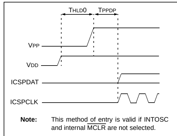
FIGURE 3-2: VDD-FIRST PROGRAM/VERIFY MODE ENTRY
