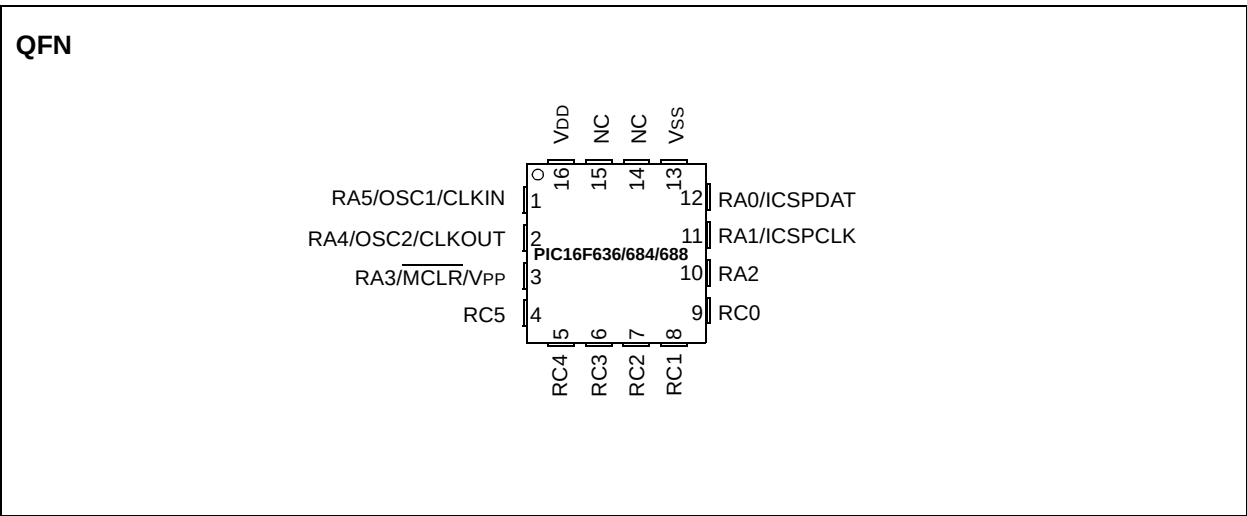
FIGURE 1-3: 16-PIN DIAGRAMS FOR PIC16F636/684/688
