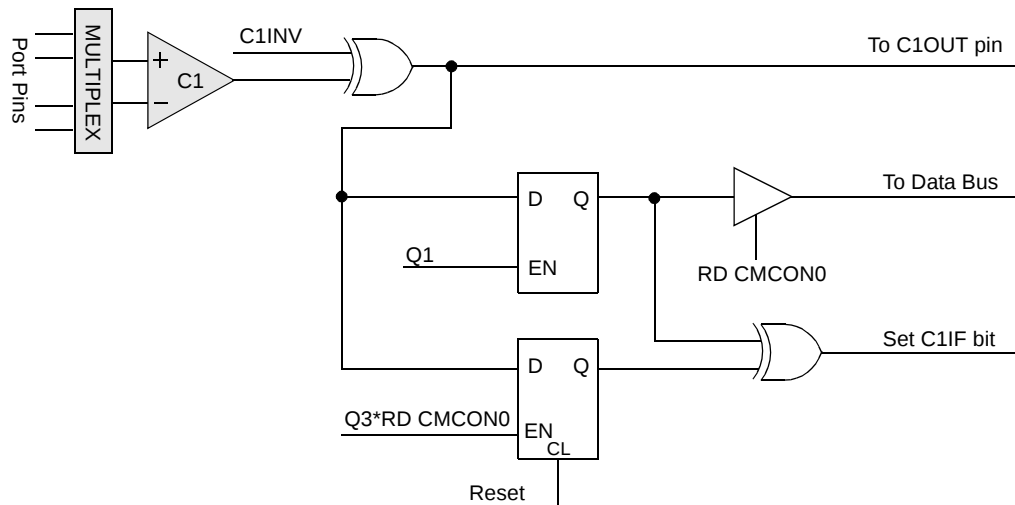
FIGURE 7-3: COMPARATOR C1 OUTPUT BLOCK DIAGRAM (PIC16F636/639)
