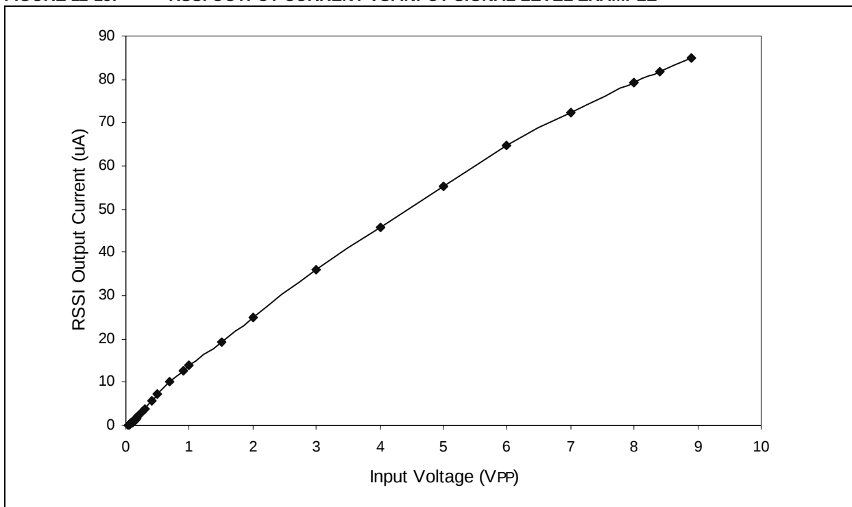
FIGURE 11-15: RSSI OUTPUT CURRENT VS. INPUT SIGNAL LEVEL EXAMPLE
