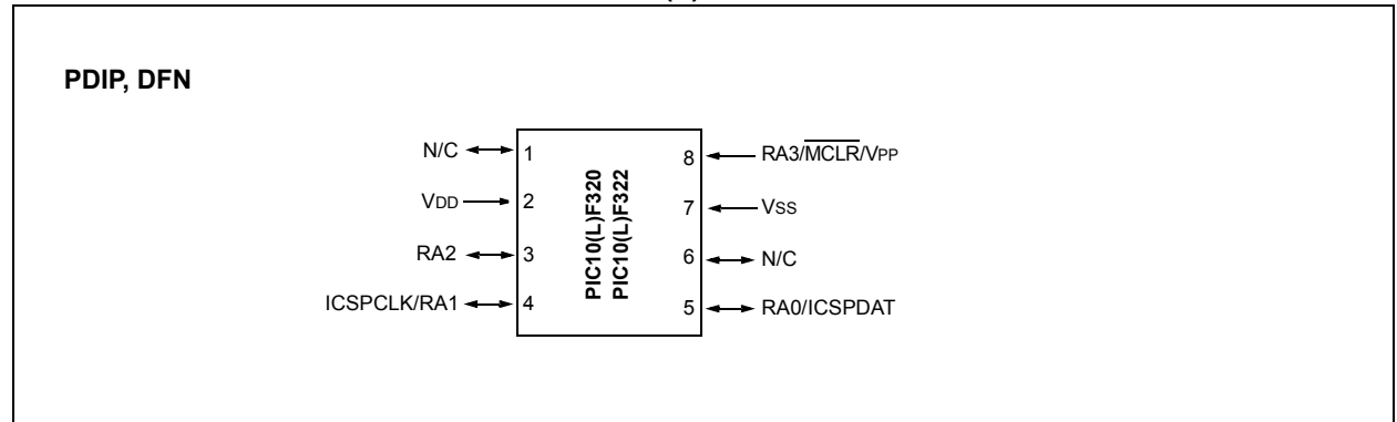
FIGURE 2-2: 8-PIN DIAGRAM FOR PIC10(L)F320/322
