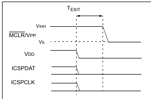
FIGURE 8-3: PROGRAMMING MODE EXIT – MCLR/VPP LAST
