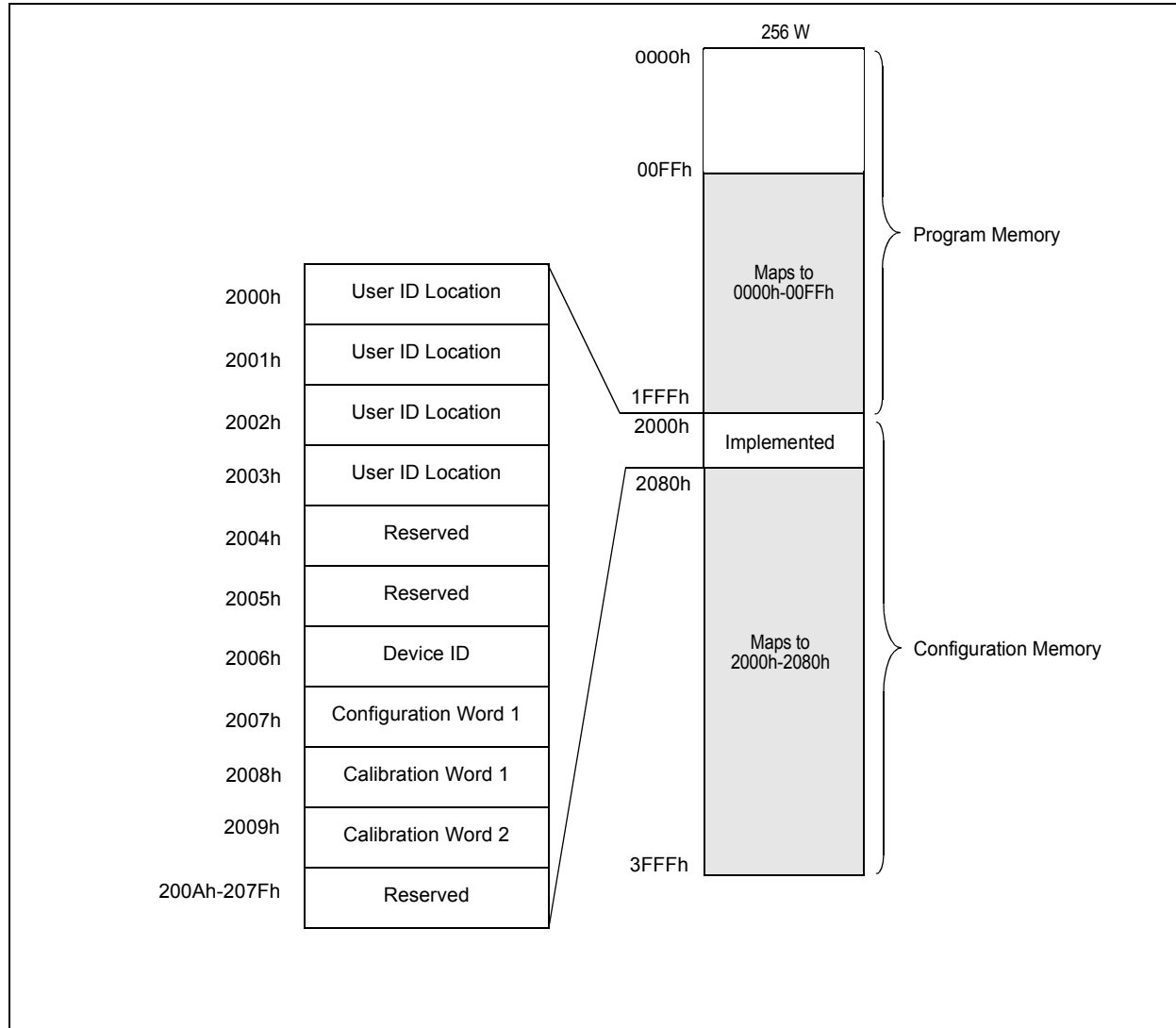
FIGURE 3-1: PIC10F320 AND PIC10LF320 PROGRAM MEMORY MAPPING
