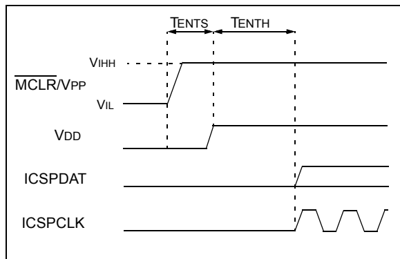
FIGURE 8-2: PROGRAMMING MODE ENTRY – MCLR/VPP FIRST
