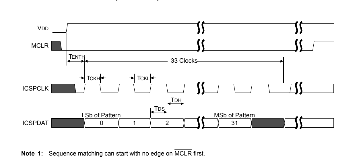
FIGURE 8-8: LVP ENTRY (POWERED)
