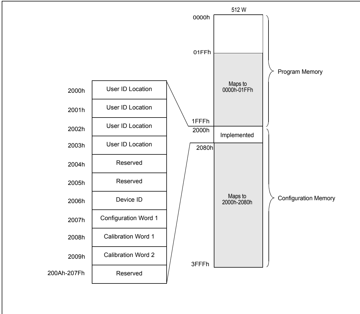
FIGURE 3-2: PIC10F322 AND PIC10LF322 PROGRAM MEMORY MAPPING
