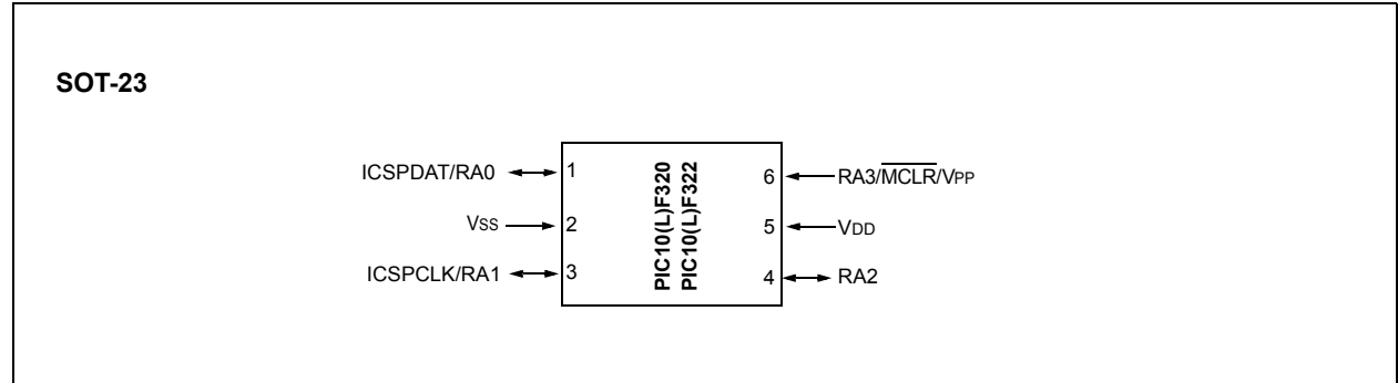
FIGURE 2-1: 6-PIN DIAGRAM FOR PIC10(L)F320/322
